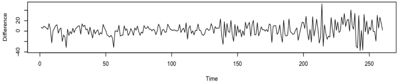
First Degree Differencing on Raw Data
