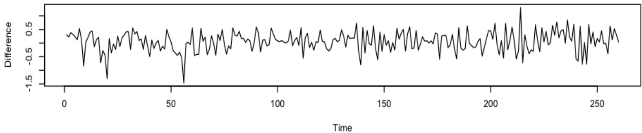
First Degree Differencing on Square-root Data
