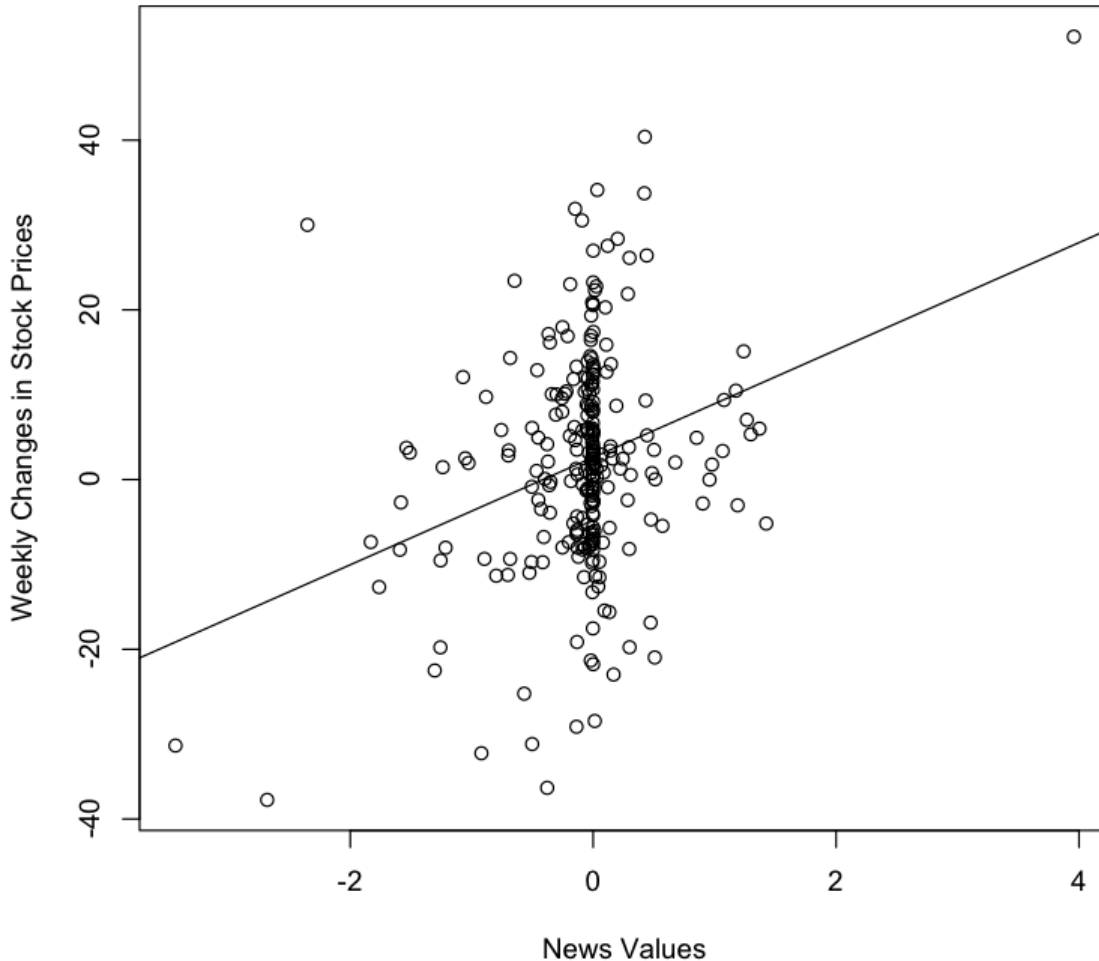
Changes in Stock Prices VS News with Regression Line
