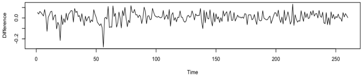
First Degree Differencing on Logged Data
