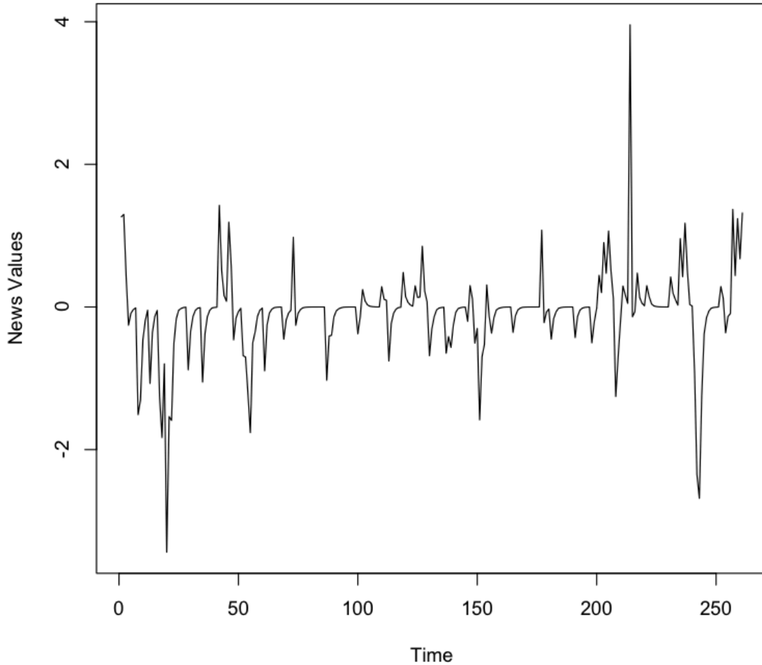
Values of News/Events over Time
