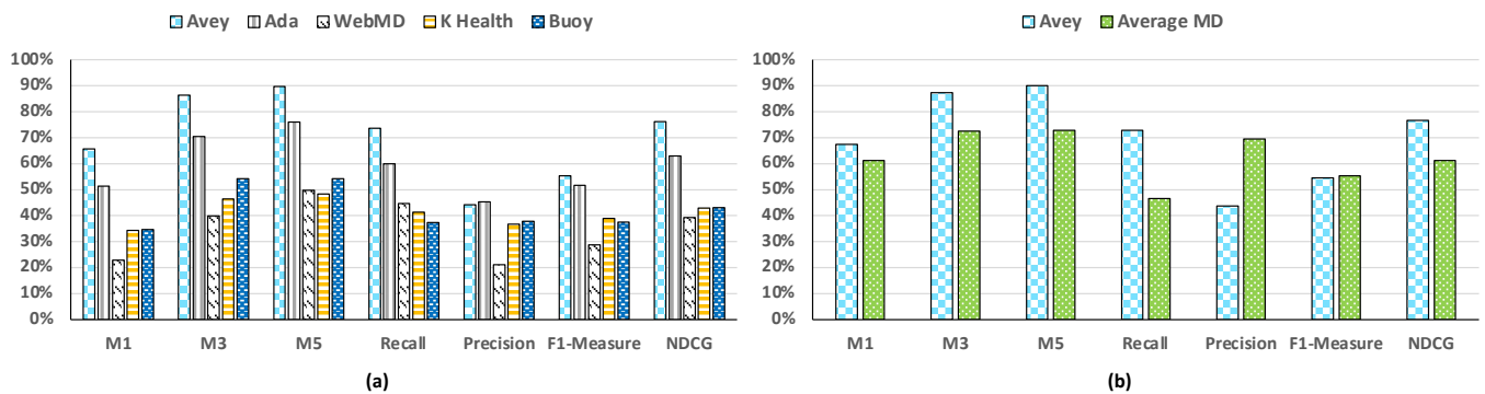
Figure 5: (a) Accuracy results considering only the succeeded vignettes with differential diagnoses across all checkers, and (b) accuracy results of Avey versus three medical doctors, on average (i.e., Average MD).
