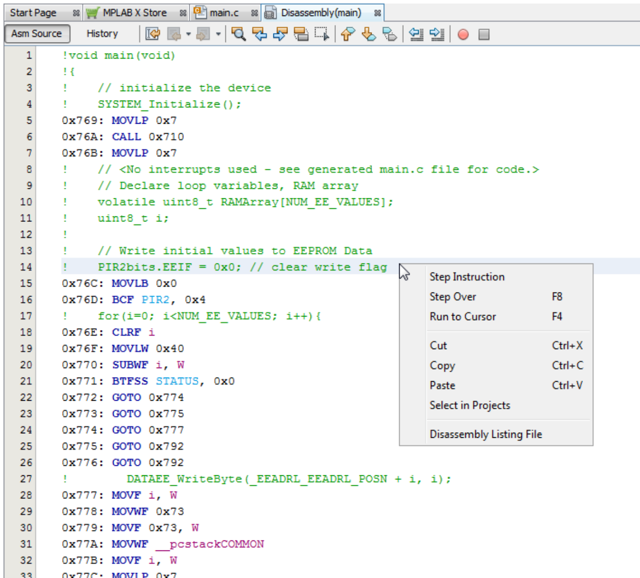
Figure 12-5. Disassembly Window
