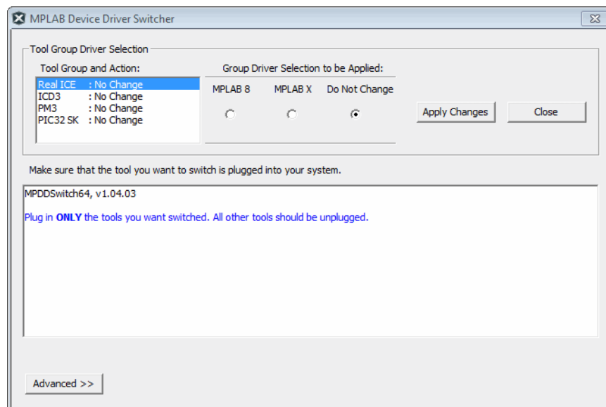
Figure 2-2. Switcher Utility
