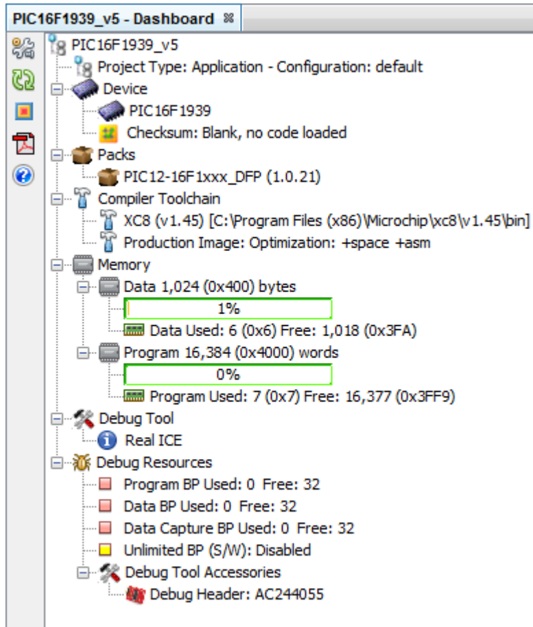
Figure 5-33. Dashboard Display
