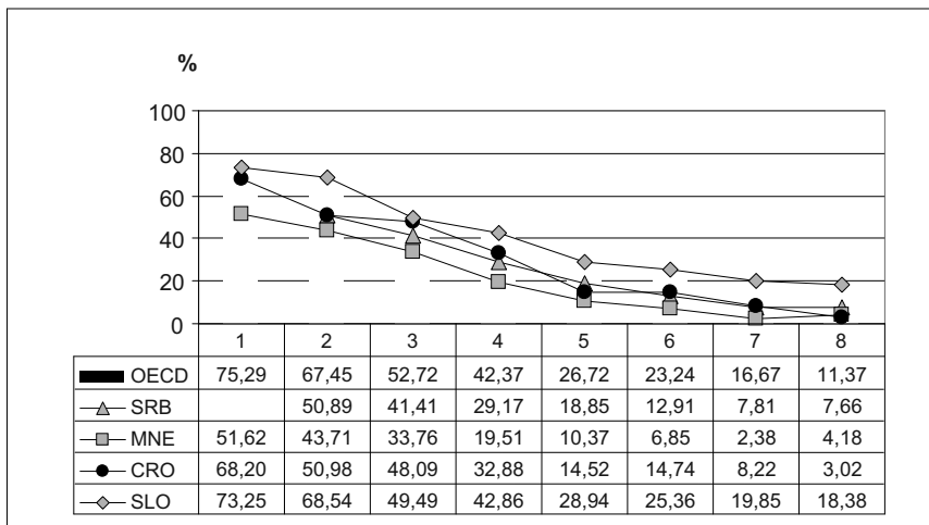
Figure 2. PISA 2009 Geometry.
