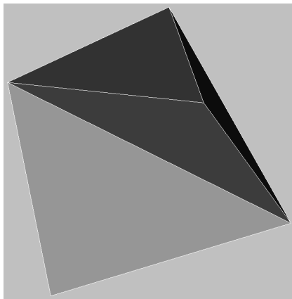
Figure 2. The 4-simplex (5-cell) with Coxeter-Schläfli symbol (3, 3, 3) .
