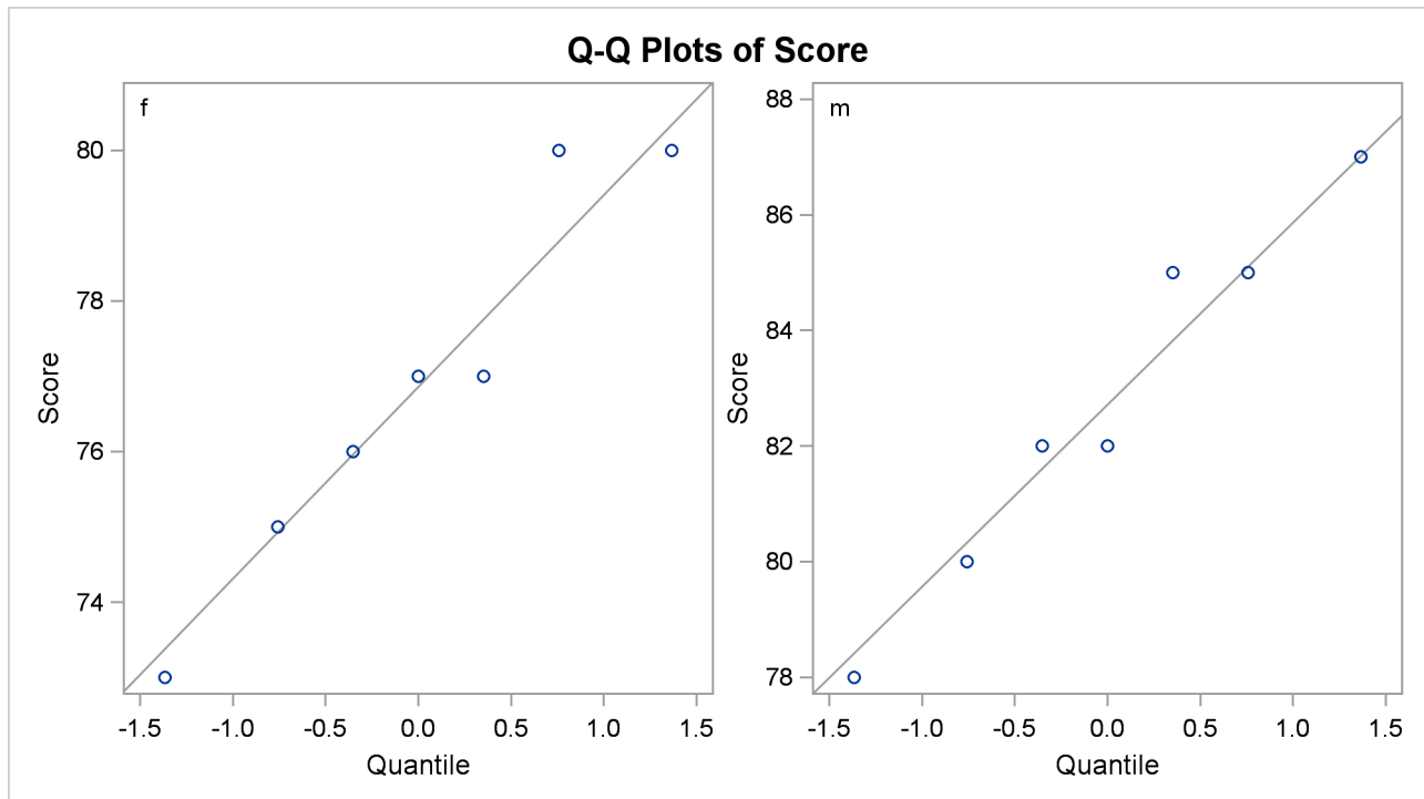
Figure 103.9 Q-Q Plot
