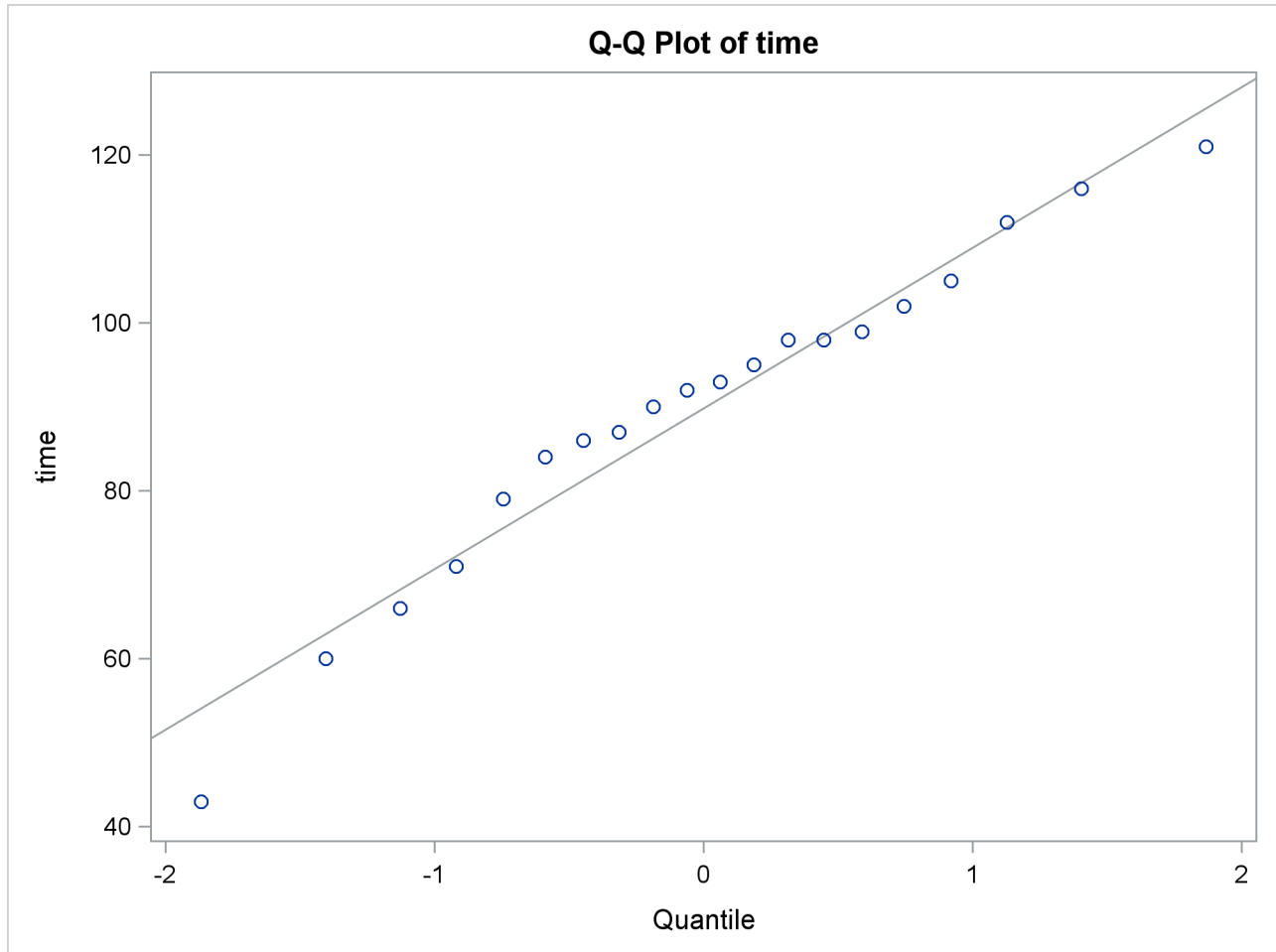
Figure 103.3 Q-Q Plot
