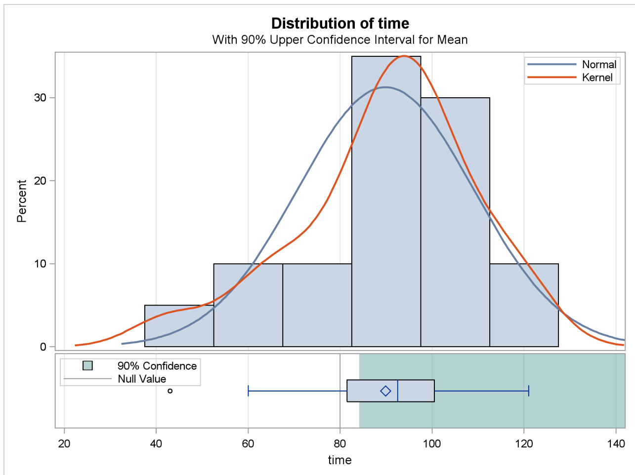
Figure 103.2 Summary Panel
