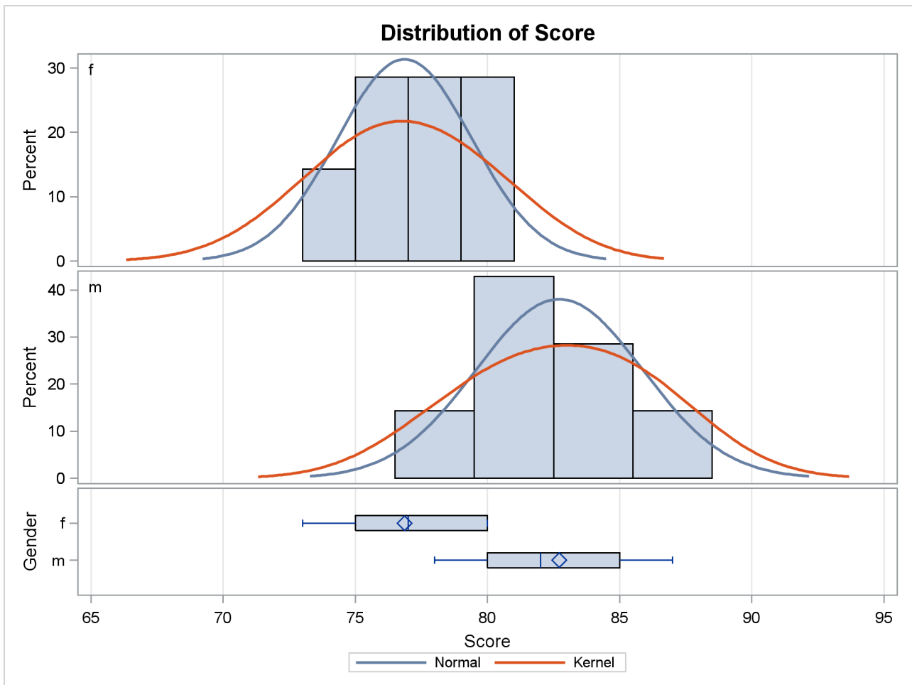
Figure 103.8 Summary Panel
