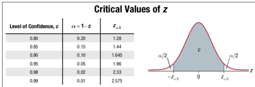
Figure 2: Z distribution2
