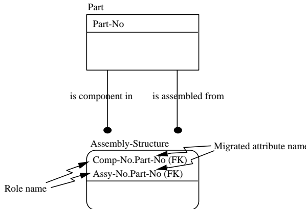
Figure 12. Role Name Syntax
