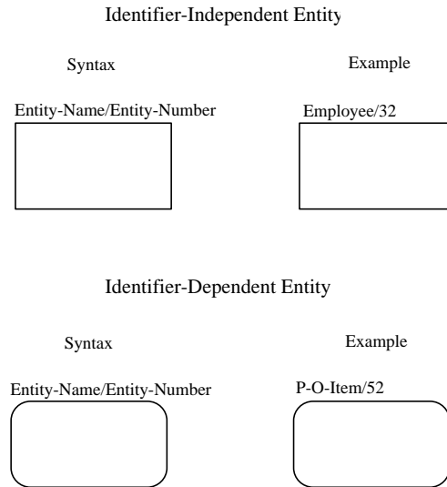
Figure 1. Entity Syntax
