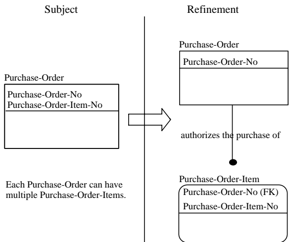
Figure A3.16. No-Repeat Rule Refinement
