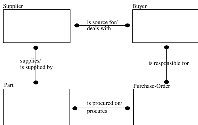
Figure A3.5. Entity Level Diagram
