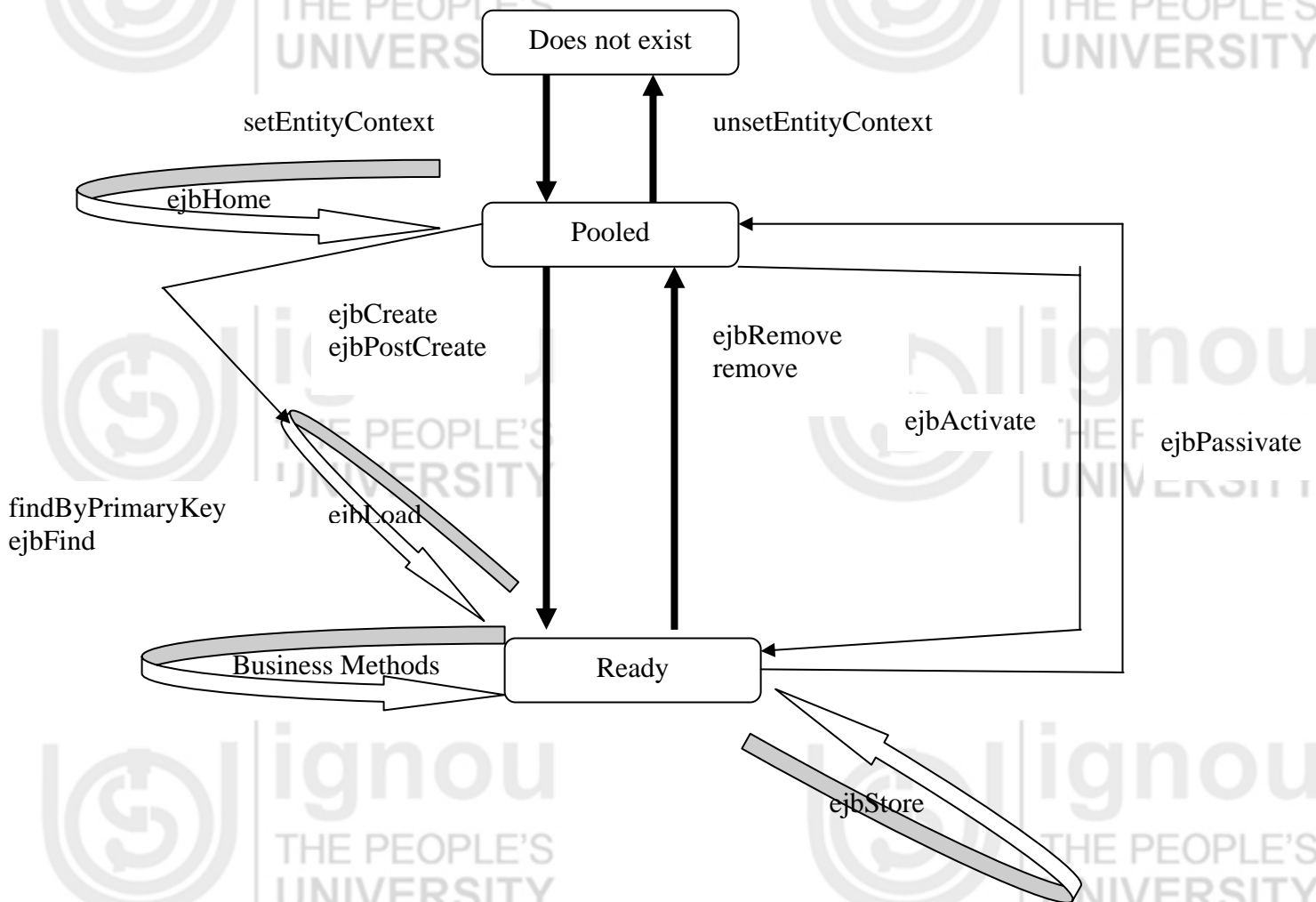
Figure 3: Life cycle of an entity bean
