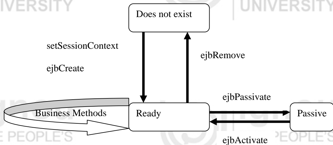
Figure 2: Life cycle of a stateful session bean
