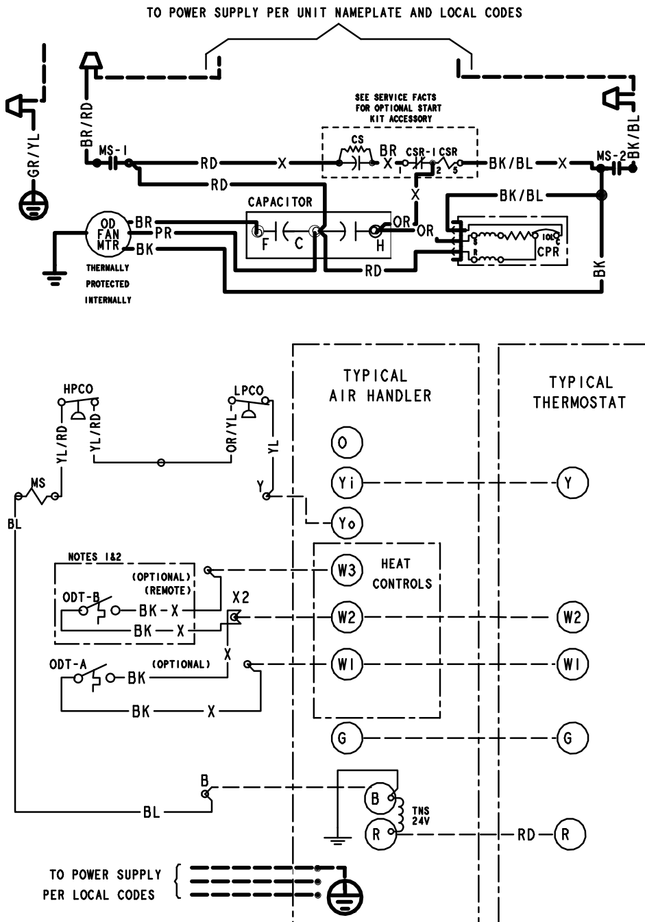
Figure 2. 5.0 Ton Models
