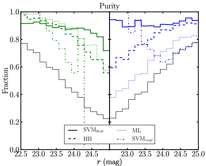
Figure 4. Similar to Figure 3 but showing purity of classified samples, instead of completeness. Results for stars are on the left in green, while those for galaxies are shown on the right in blue. Here, SVM algorithms generally outperform all others, if given a very good set of training data ( SVM_{best} ). For stars, our HB algorithm delivers somewhat similar purity to the SVM_{best} scenario. For galaxies, however, HB underperforms SVM_{best} as the stellar fraction of the sample decreases.
