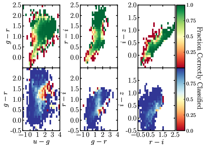
Figure 6. Same as Figure 5, but for an SVM trained with data that span the S/N range of the whole sample ( SVM_{best} ). The top panel shows the performance on stars, and the bottom panel shows the performance on galaxies. By inspection, it is clear that SVM_{best} outperforms HB template fitting, particularly in the case of galaxies. A striking difference is the poor galaxy classification of HB compared to SVM_{best} in u-g . This may indicate a model deficiency in the u spectral range of our galaxy templates.
