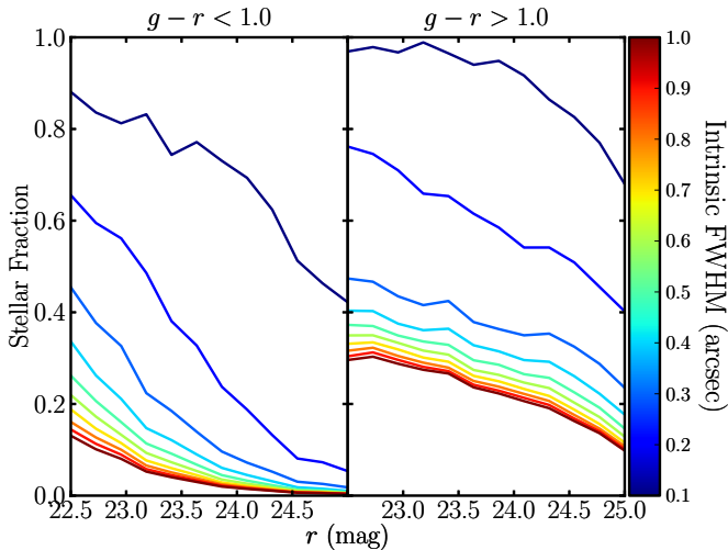
Figure 1. Stellar fraction of COSMOS sources as a function of magnitude, for sources with g-r < 1 (left) and g-r > 1 (right). Only stars and galaxies were included in this figure. Only a few percent of the COSMOS point sources are AGNs. Colored curves indicate the upper limit in intrinsic FWHM allowed in the sample. Even in an optimistic scenario where galaxies with \text{FWHM} \gtrsim 0.2 arcsec can be morphologically distinguished from stars, unresolved galaxies will far outnumber stars in point-source catalogs at faint magnitudes. This challenge is much greater for blue stars than for red stars.
