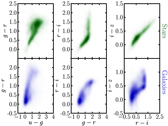
Figure 2. Color-color space distribution of point sources (FWHM < 0.2 arcsec) in the COSMOS catalog. It is clear that stars in the sample follow a tight locus in all slices of color-color space, while galaxies are more generally distributed. Even so, comparison by eye reveals significant overlap between stars and galaxies, particularly for bluer sources.
