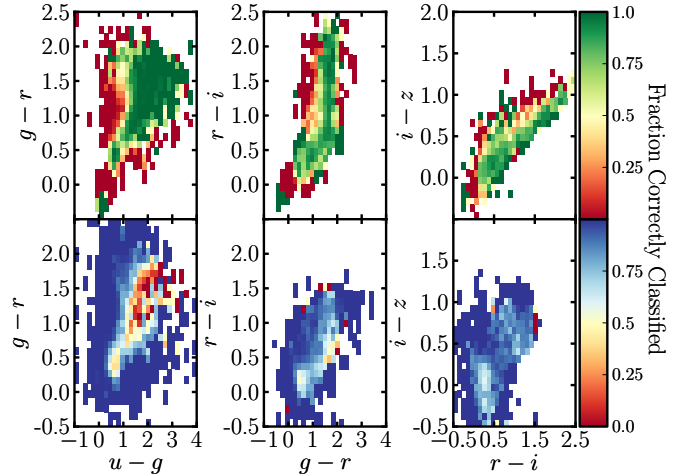
Figure 5. Fraction of objects correctly classified at \ln(\Omega) = 0 using our HB template fitting, distributed in ugriz color-color space. The top panel shows the performance on stars, and the bottom panel shows the performance on galaxies. Comparing with Figure 2, it is clear that classification is most successful for regions in which stars and galaxies do not overlap in color-color space.
