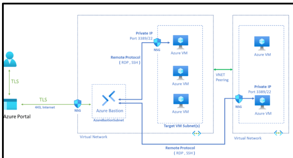
Figure 23 – Azure Bastion Host 19
