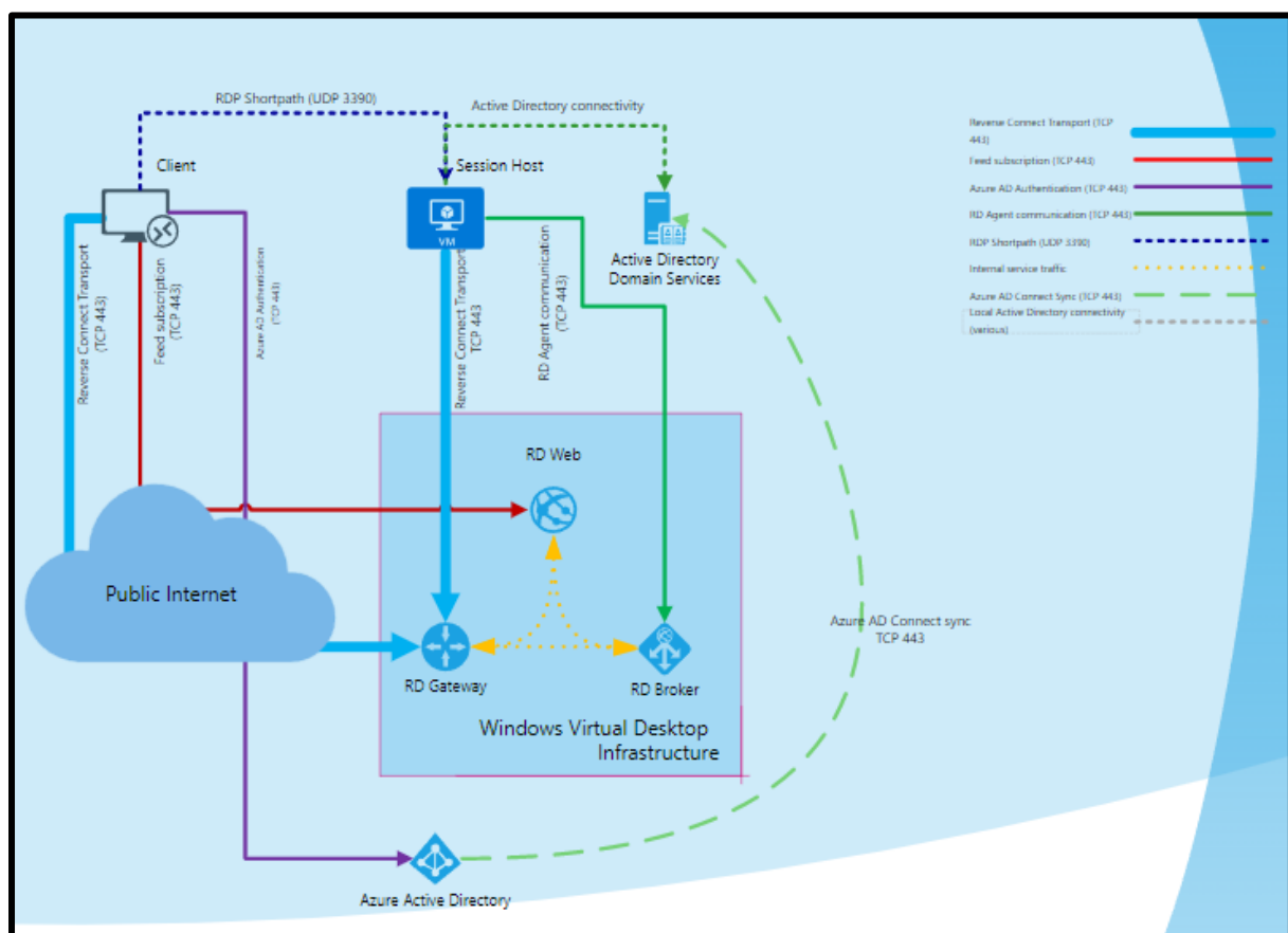
Figure 6 – RDP Shortpath Network Connections 4
