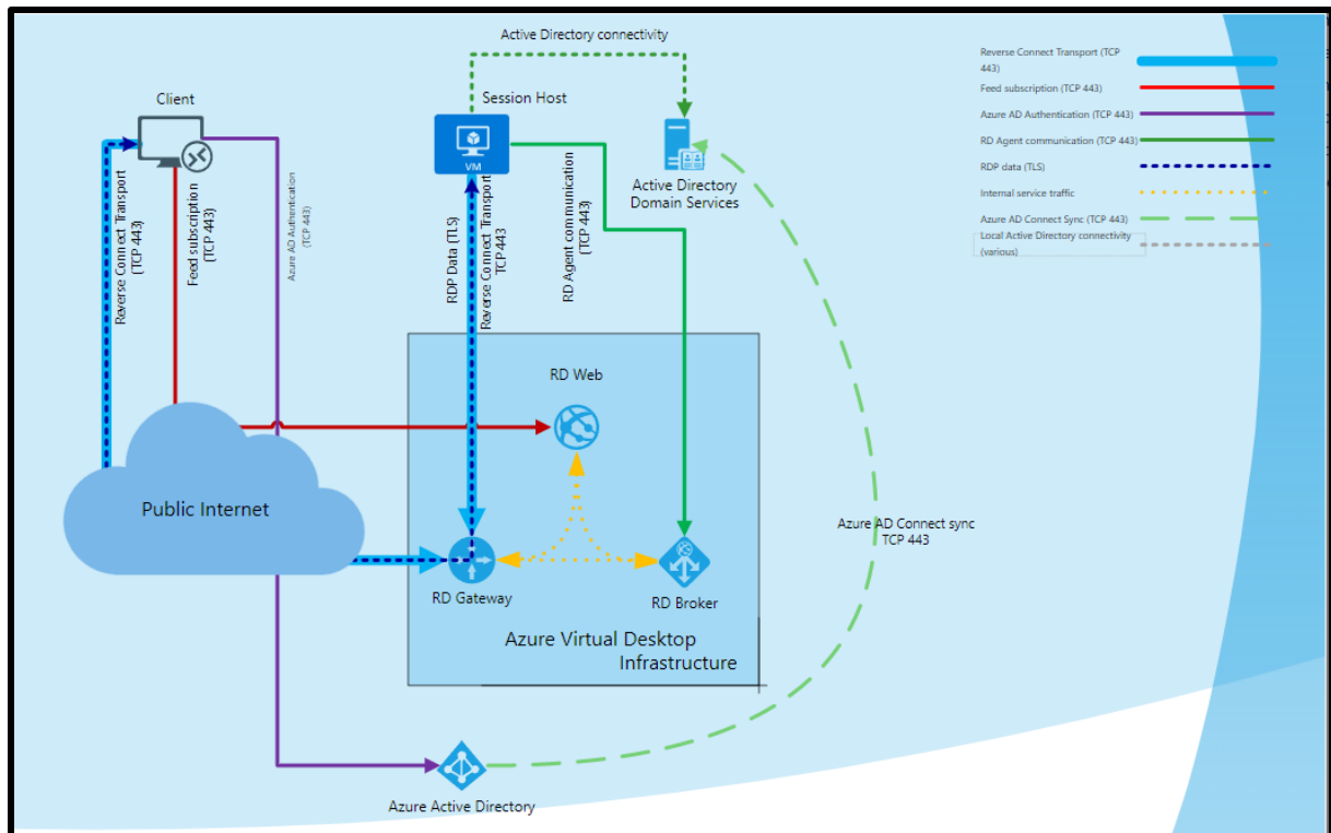
Figure 5 - Azure Virtual Desktop Network Connectivity 3
