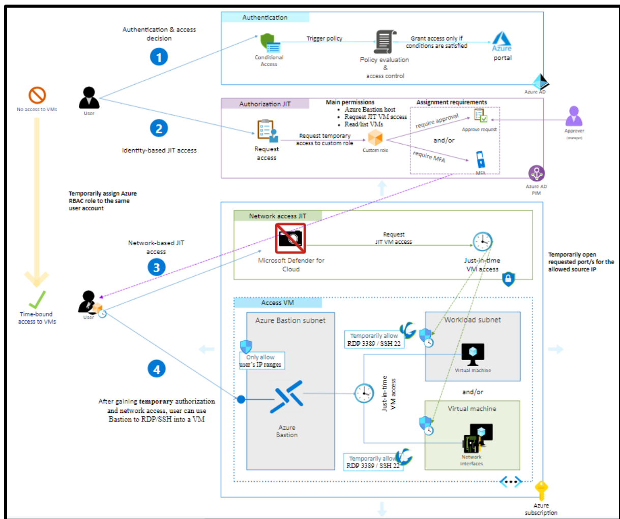
Figure 12 - Multi-layered Protection for Azure VM 9
