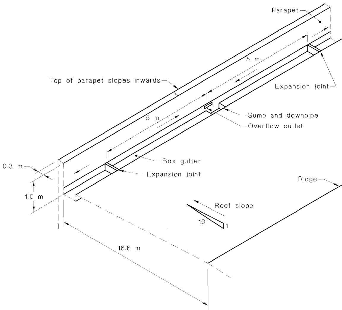
FIGURE J3 ROOF PLAN
