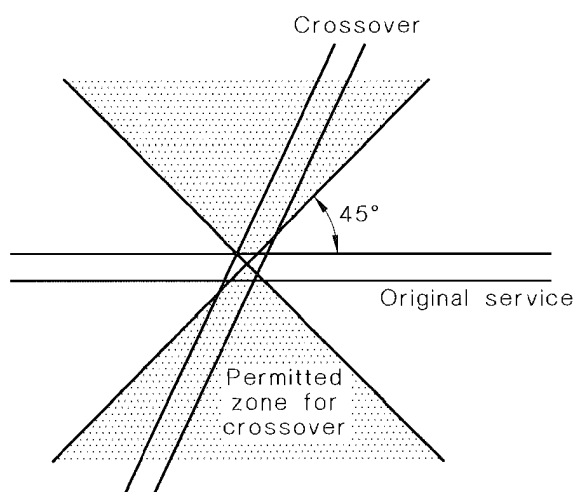
FIGURE 7.2 PERMITTED CROSSOVER ZONE FOR ELECTRICAL CABLES AND GAS PIPES
