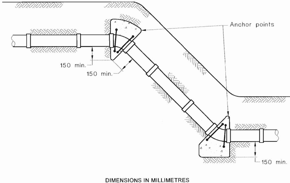
FIGURE 8.10 ANCHORING OF SITE STORMWATER DRAINS
