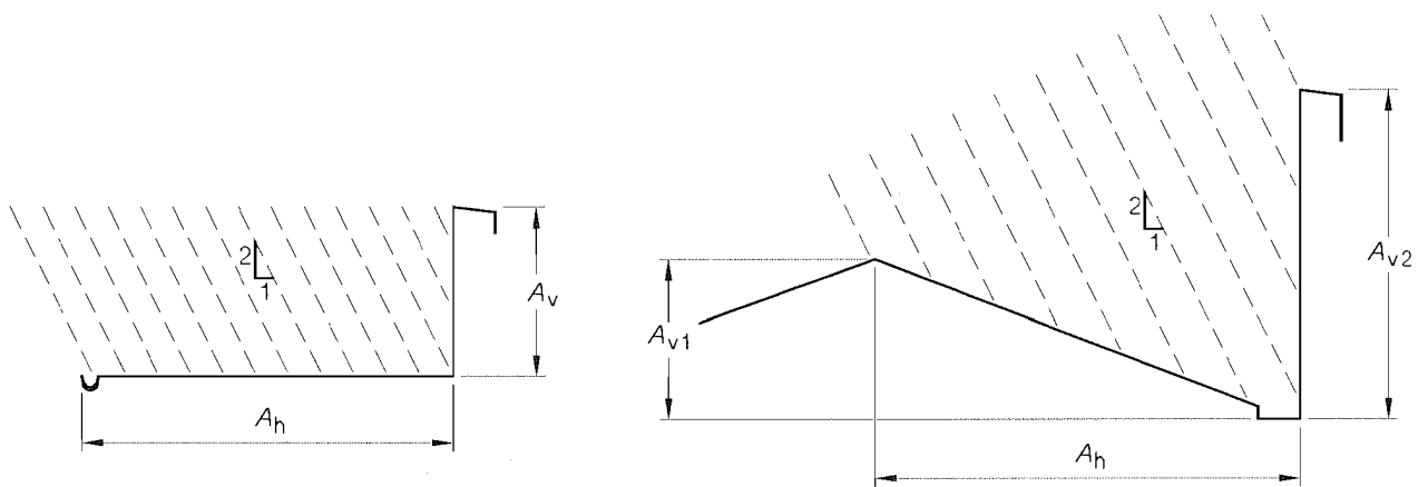
(a) Vertical wall with flat roof
