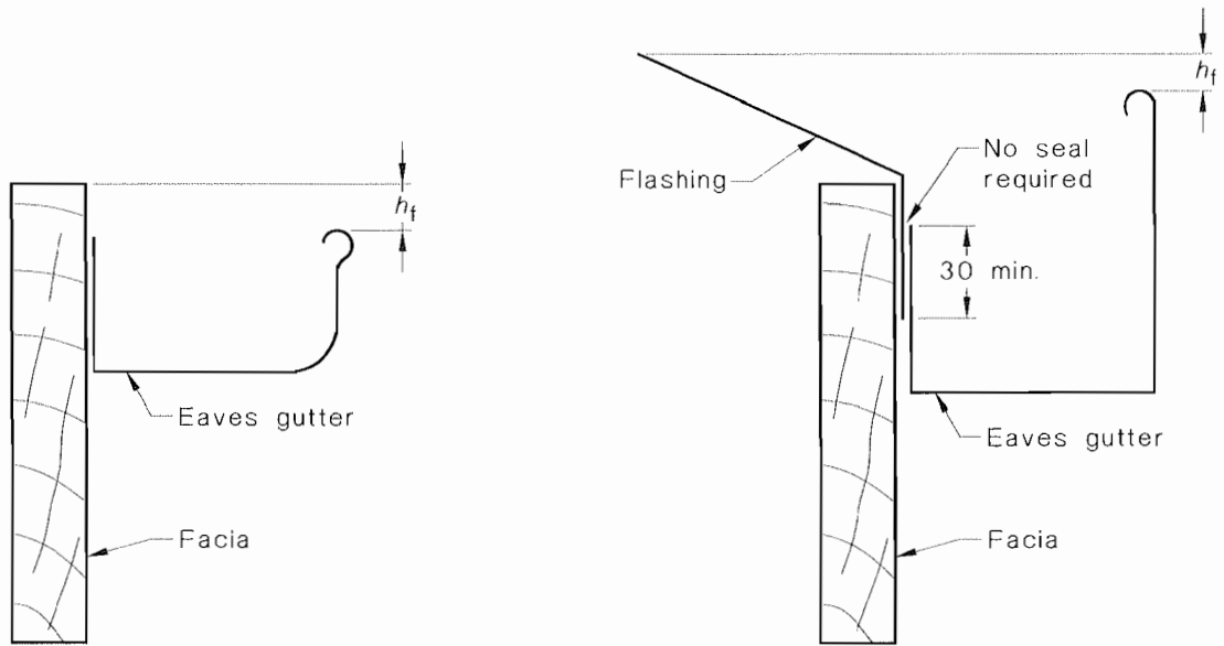
(a) Eaves gutter with low front
