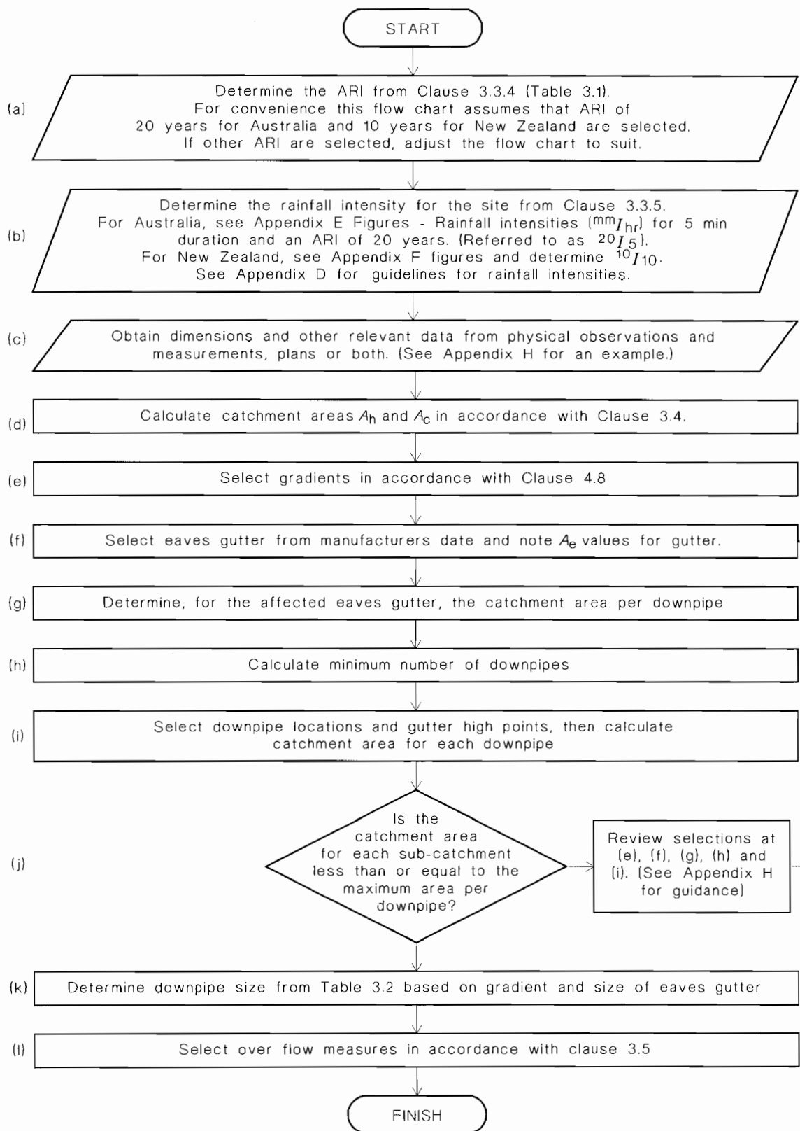
FIGURE 3.4 (in part) FLOW CHART—GENERAL METHOD FOR DESIGN OF EAVES-GUTTER SYSTEMS
