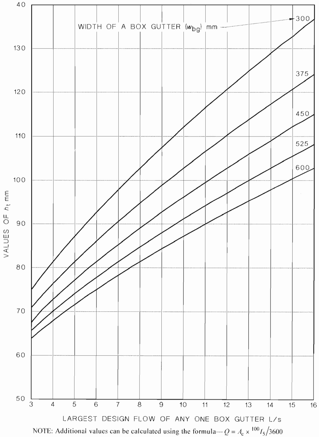
FIGURE 18 DESIGN GRAPH FOR SUMP/HIGH-CAPACITY OVERFLOW DEVICE
