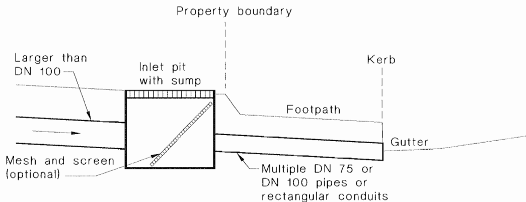
FIGURE 8.1 TYPICAL ARRANGEMENT OF INLET PIT AND FOOTPATH CROSSING
