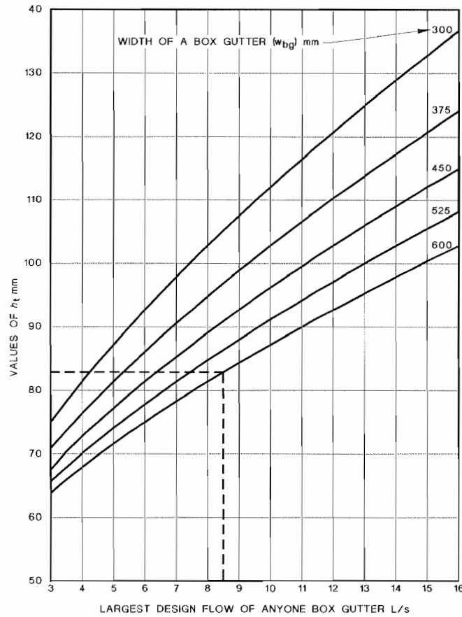
FIGURE 18 REQUIRED SIZE OF SUMP/HIGH-CAPACITY OVERFLOW DEVICE
