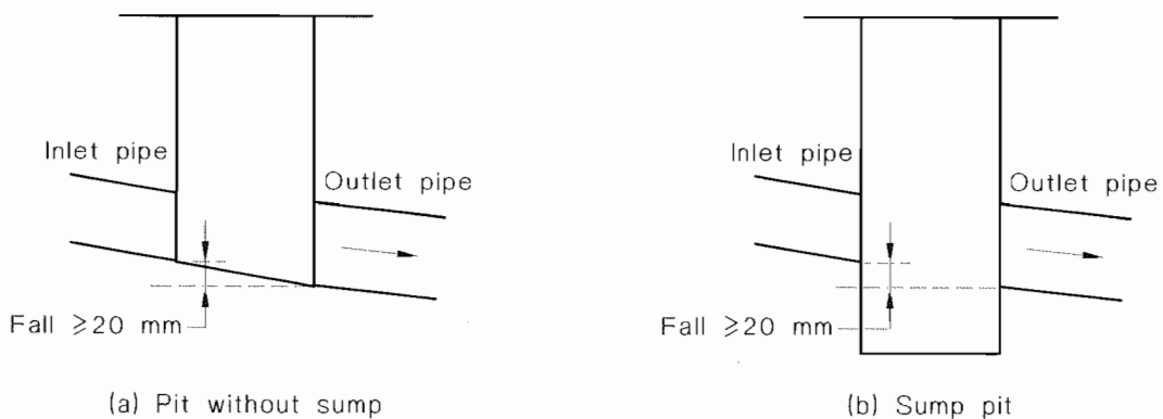
FIGURE 8.4 PIT ARRANGEMENTS
