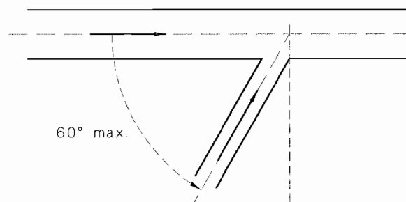
FIGURE 8.6 ALLOWABLE OBLIQUE OR SWEEP JUNCTION CONNECTION
