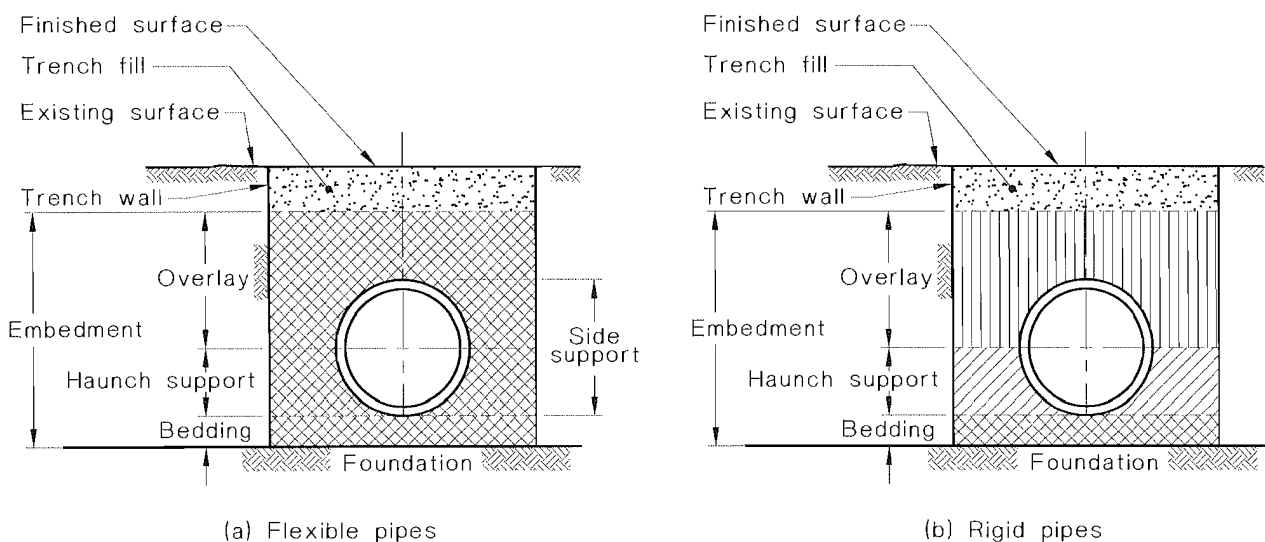
FIGURE 7.1 TRENCH TERMINOLOGY
