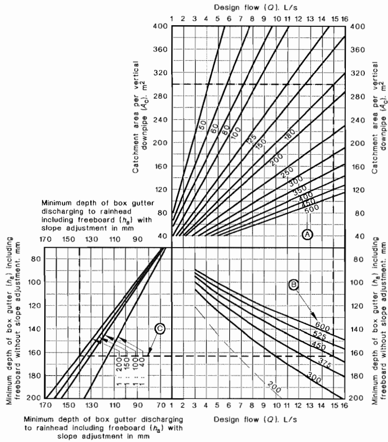
FIGURE 11 REQUIRED SIZE OF BOX GUTTER DISCHARGING TO A RAINHEAD (a) Application of Figure 11
