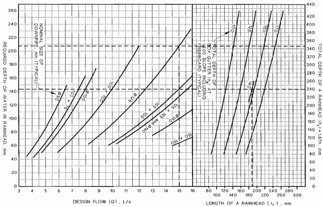
FIGURE 13 DESIGN GRAPH FOR RAINHEAD (b) Application of Figure 13
