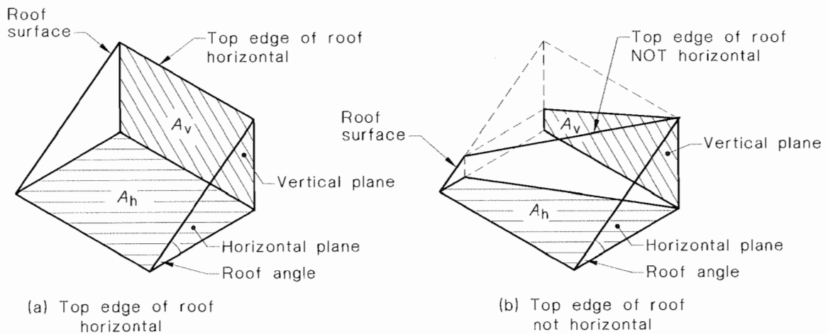
FIGURE 3.1 COMPONENTS OF THE CATCHMENT AREA
