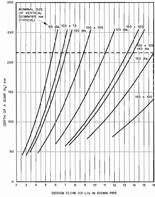
FIGURE 14 DESIGN GRAPH FOR SUMP
