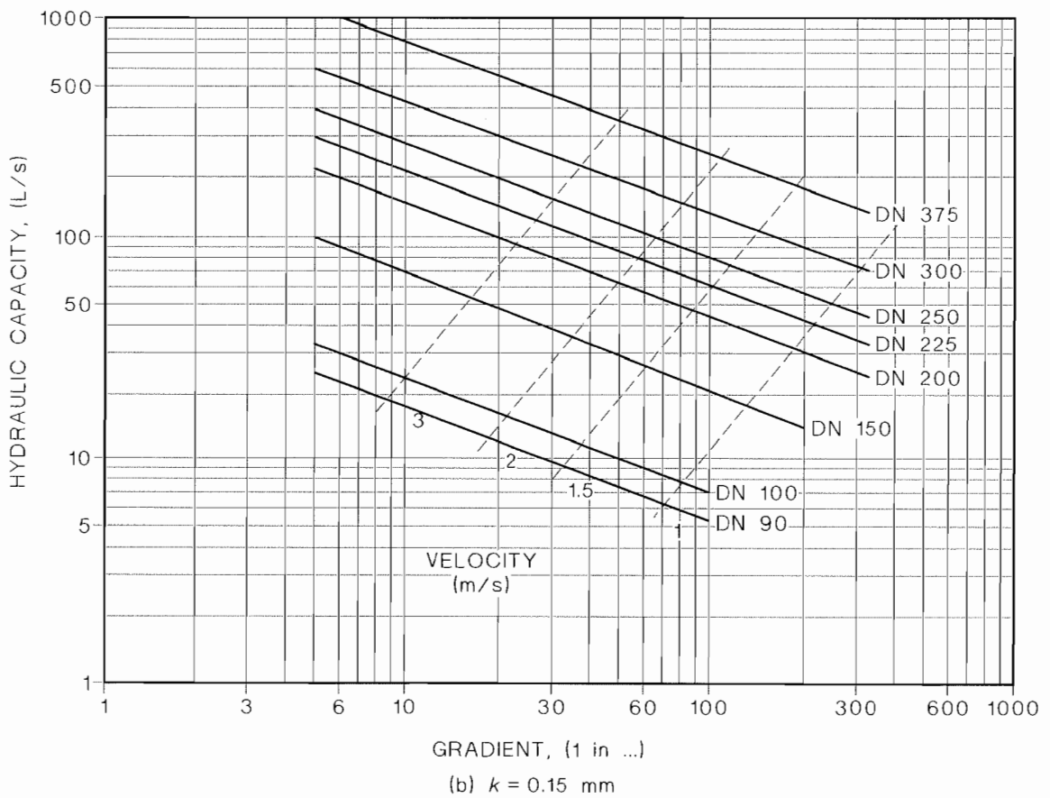
FIGURE 5.1 (in part) HYDRAULIC DESIGN CHARTS—WATER AT 20°C
