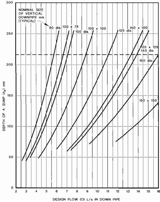
FIGURE I4 DESIGN GRAPH FOR SUMP
