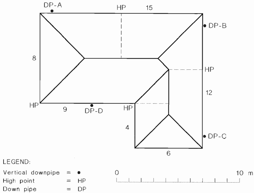
FIGURE H3 ROOF PLAN—CASE 1
