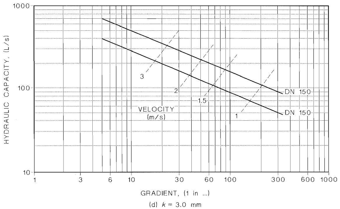
FIGURE 5.1 (in part) HYDRAULIC DESIGN CHARTS—WATER AT 20°C
