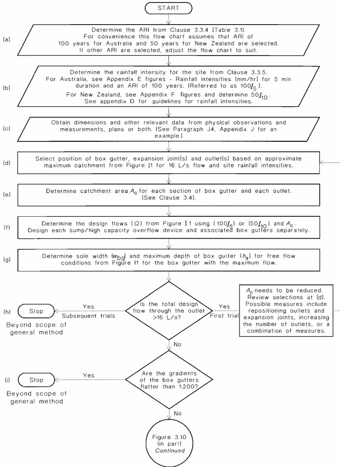
FIGURE 3.10 (in part) FLOW CHART—GENERAL METHOD FOR DESIGN OF BOX GUTTERS, SUMP/HIGH-CAPACITY OVERFLOW DEVICES AND DOWNPIPES
