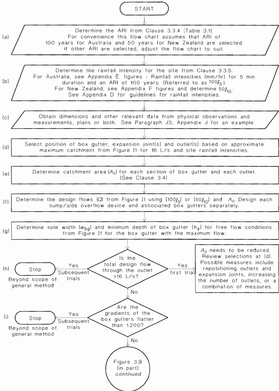
FIGURE 3.9 (in part) FLOW CHART—GENERAL METHOD FOR DESIGN OF BOX GUTTERS, SUMP/SIDE OVERFLOW DEVICES AND DOWNPIPES
