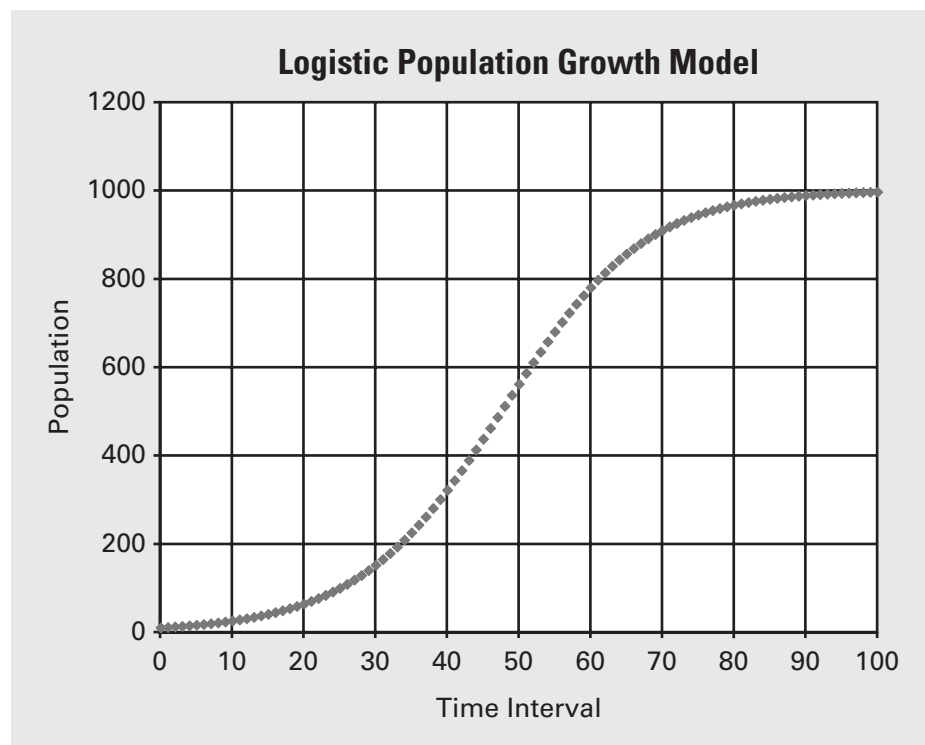
Figure 21. A Discrete Logistic (S-shaped) Growth Model
