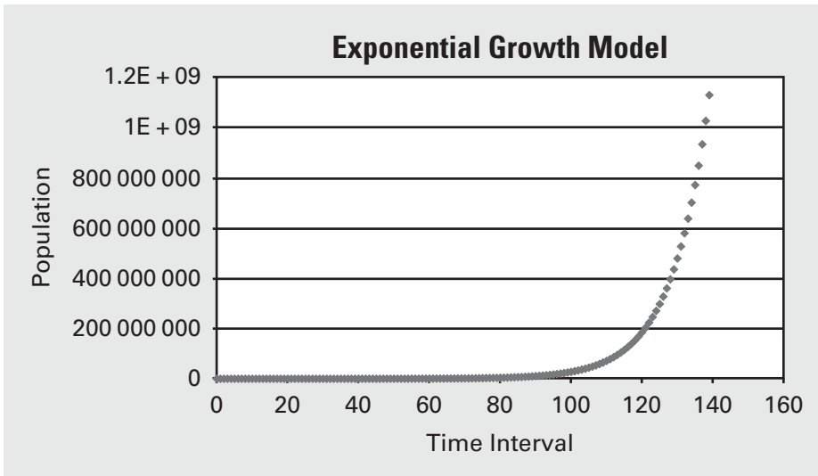
Figure 20. Exponential Growth Model
