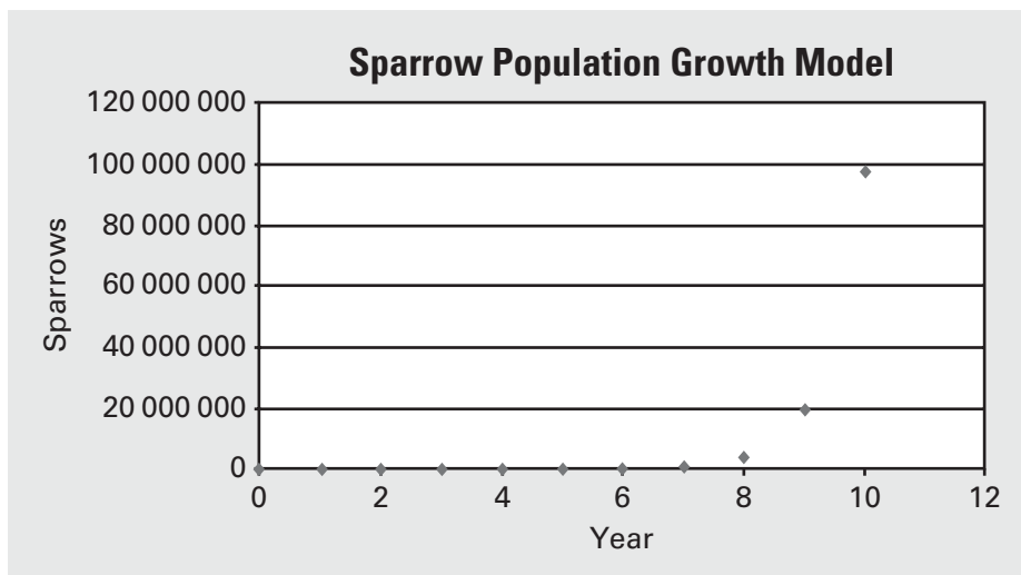
Figure 18. Standard x - y Scatterplot for Sparrow Population Growth Model
