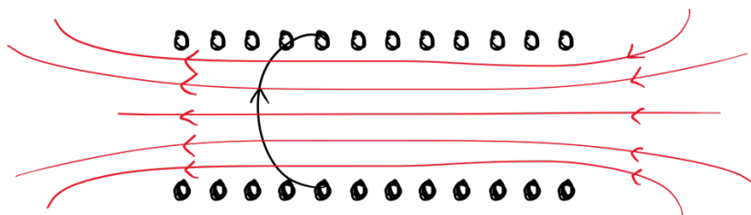
Magnetic field pattern due to current in long solenoid
