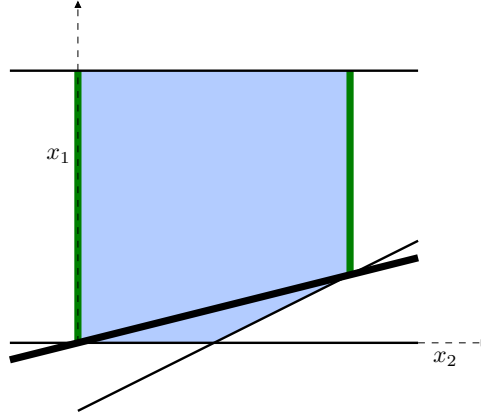
Figure 13: Mixed-integer rounding (MIR) cut. Feasible set of the LP relaxation (hatched), integer feasible set (bold black lines), and MIR cut (grey) x_2 \leq 2x_1 + \frac{1}{2} derived from the inequality x_2 \leq \frac{1}{2} + x_1 .
