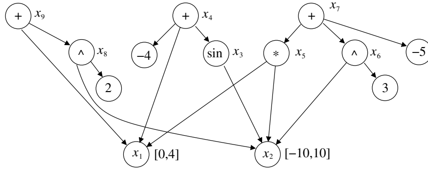
Figure 23: Association between auxiliary variables and the nodes of the DAG related with the problem in (5.9).
