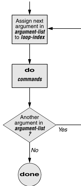
Figure 10-4 A for...in flowchart
