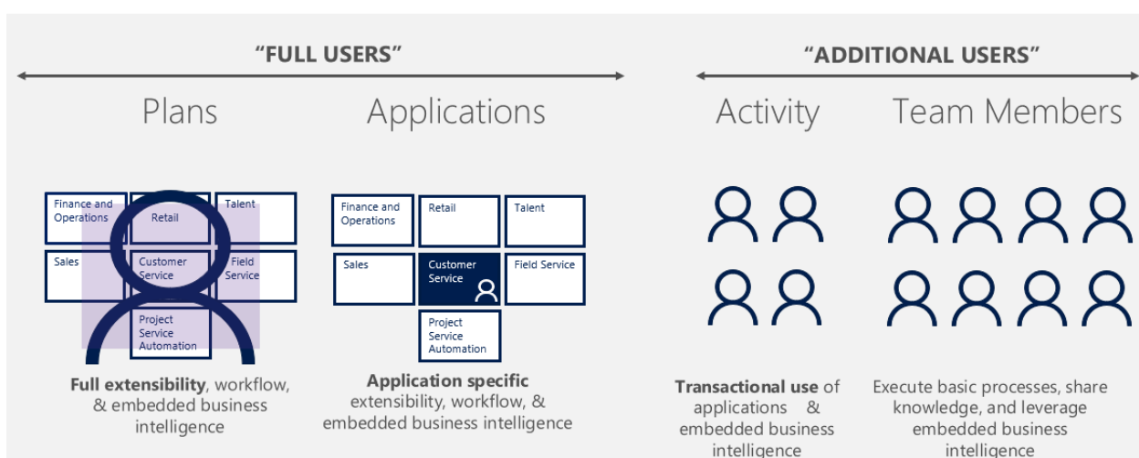
Figure 7: User Types
