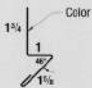
13 - Rat Guard
