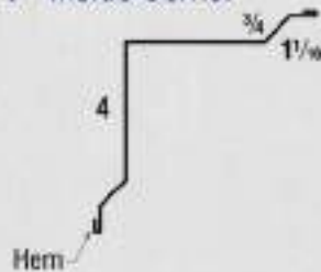
4 - Inside Corner
