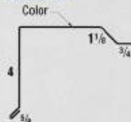
10 - Gable Trim
