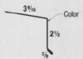
8 - Eave Drip Trim
