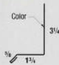
11 - Drip Cap
