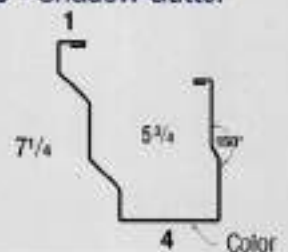
16 - Shadow Gutter
