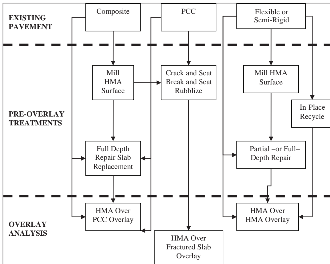
Figure 13-2. Flow Chart of Rehabilitation Design Options Using HMA Overlays
