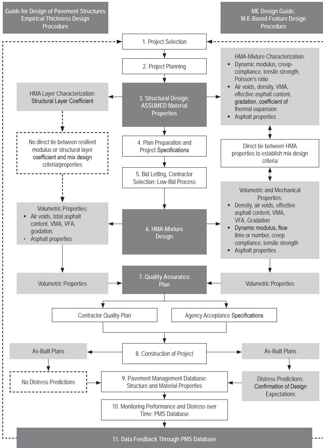
Figure 1-2. Typical Differences Between Empirical Design Procedures and an Integrated M-E Design System, in Terms of HMA-Mixture Characterization
