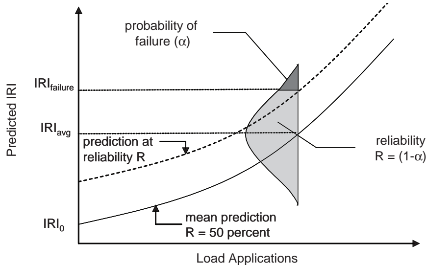
Figure 8-1. Design Reliability Concept for Smoothness (IRI)
