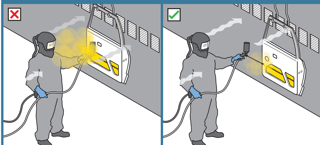
FIGURE 3: The Spraying with a 'short' nozzle may cause overspray of the operator.
