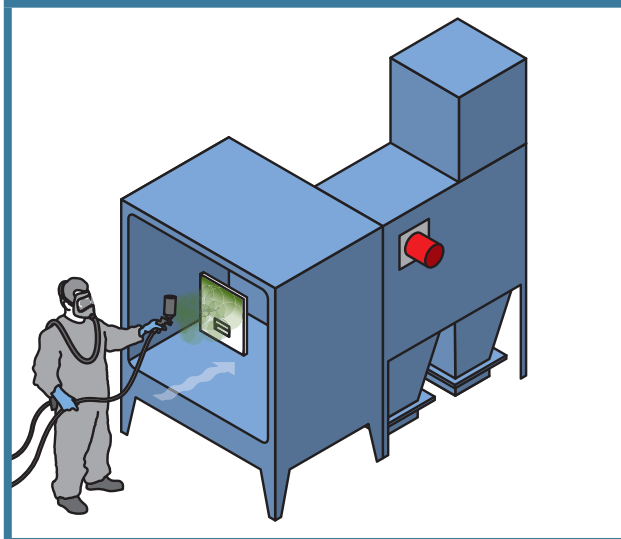
FIGURE 10: Example of a local exhaust ventilation system suitable for powder coating activities
