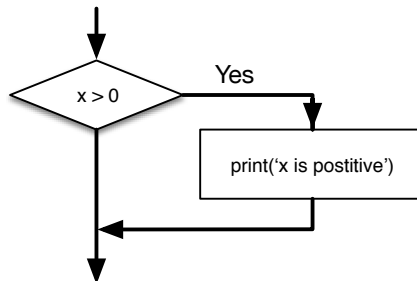
Figure 3.1: If Logic
