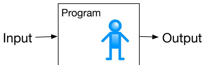
Figure 14.1: A Program
