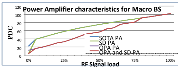
FIGURE 23. BS Power Consumption, Analysis and Optimization Tool
