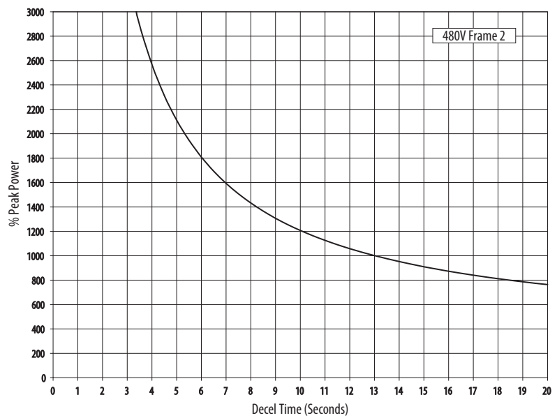
Figure 17 - PowerFlex 700 – 480 Volt, Frame 2
