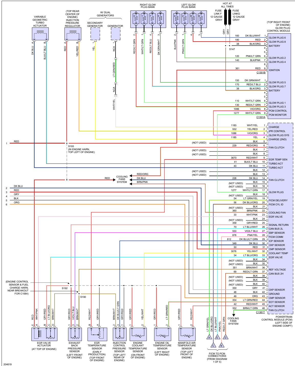
Fig 5: 6.0L Diesel, Engine Performance Circuit (5 of 5)
