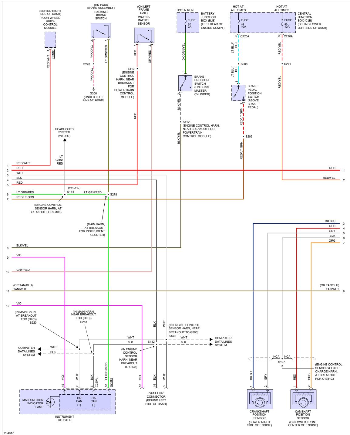
Fig 3: 6.0L Diesel, Engine Performance Circuit (3 of 5)
