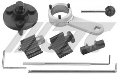
JTC-4330 VAG ENGINE TIMING TOOL SET (TDI)
