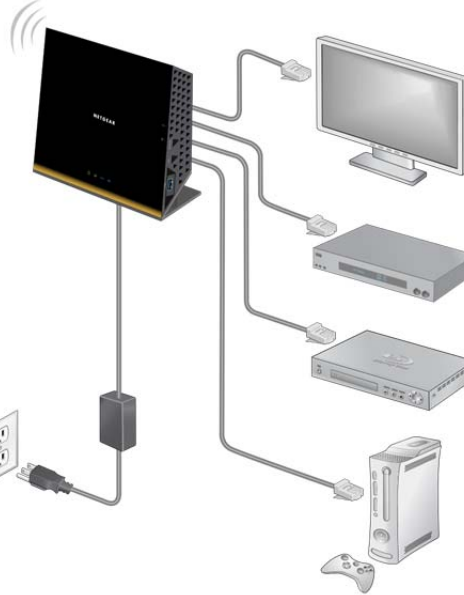
Figure 8. Router in bridge mode with an 802.11ac WiFi connection
