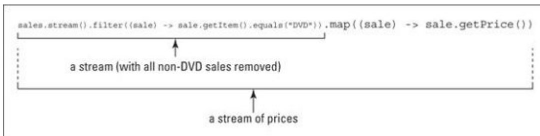
FIGURE 12-13: Getting the price from each DVD sale.
