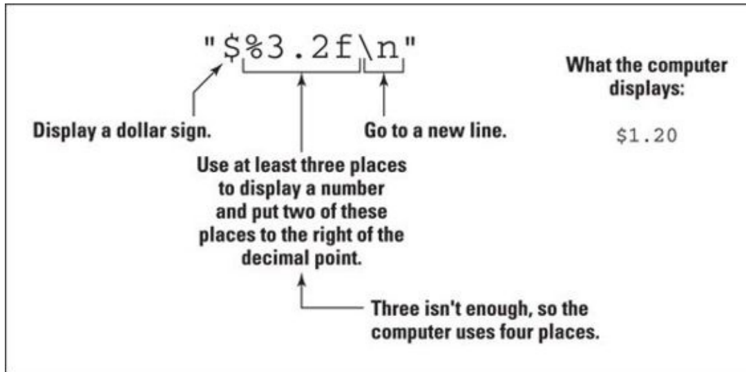
Figures 7-13: Specifying too few places to display a value.
