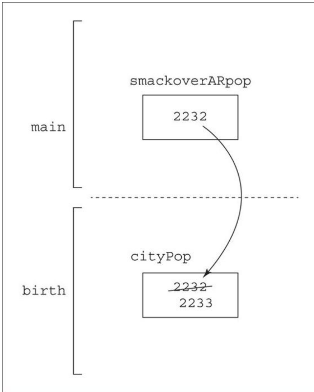
FIGURE 10-11: Pass by value, under the hood.
