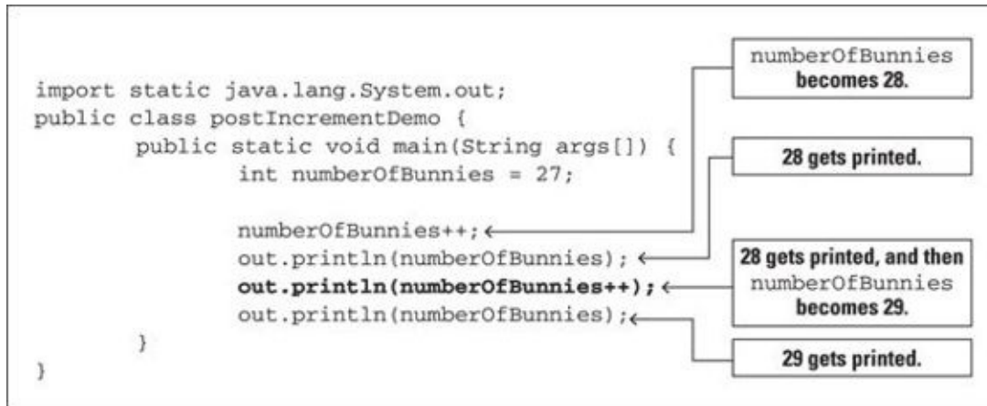
FIGURE 4-15: Using postincrement.
