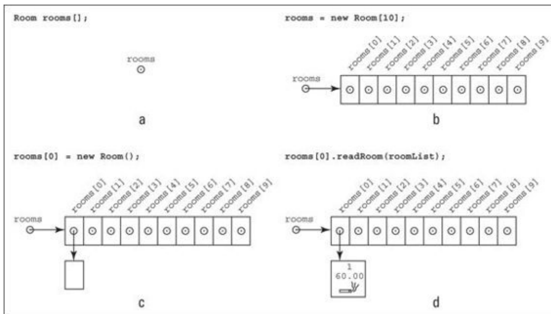
FIGURE 11-11: Steps in creating an array of objects.
