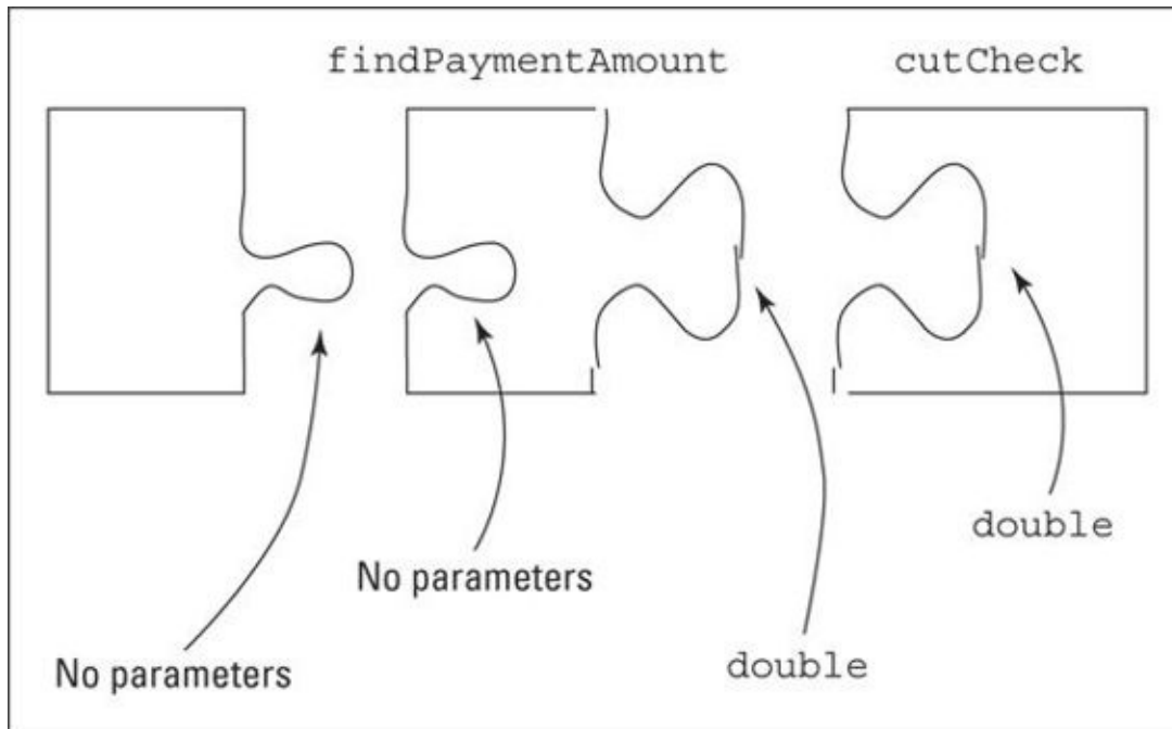
FIGURE 8-7: Matching parameters.
