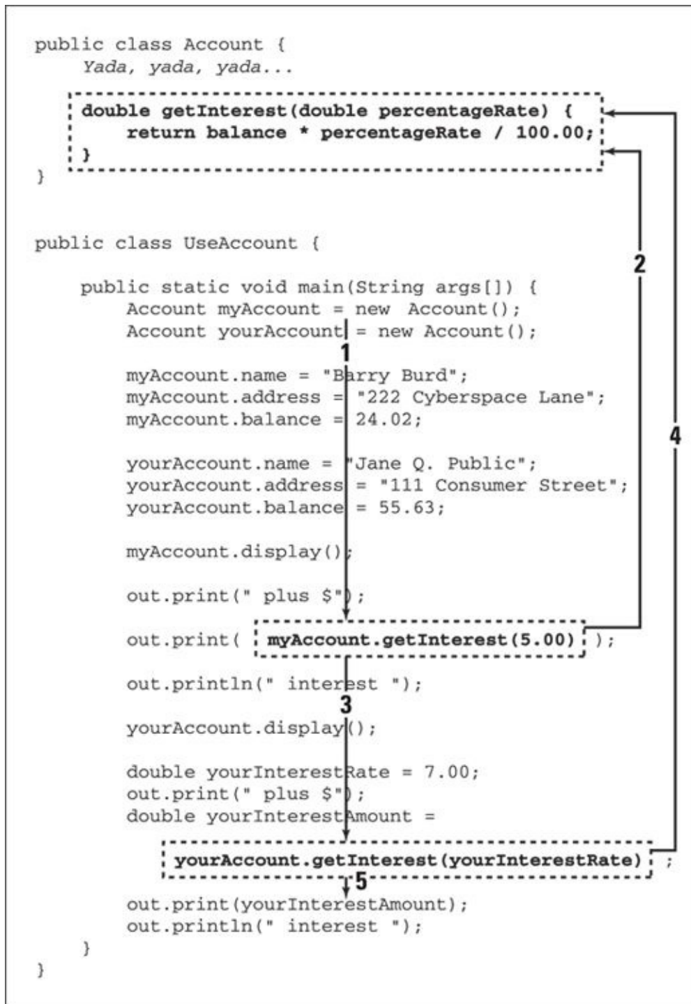
FIGURE 7-7: The flow of control in Listings 7-5 and 7-6.
