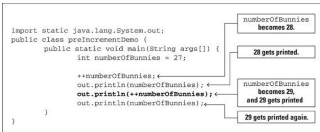
FIGURE 4-13: Using preincrement.
