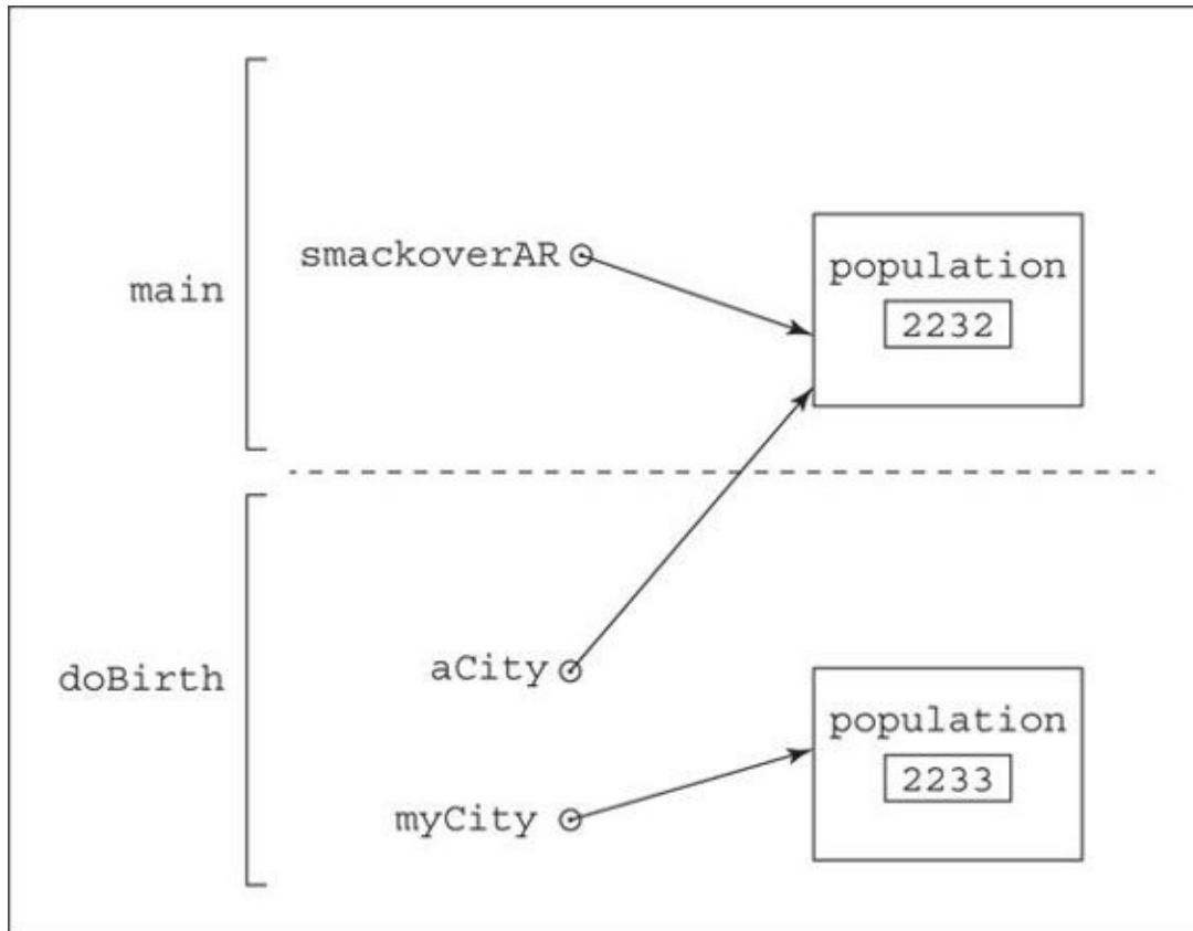
FIGURE 10-13: The doBirth method creates a City instance.
