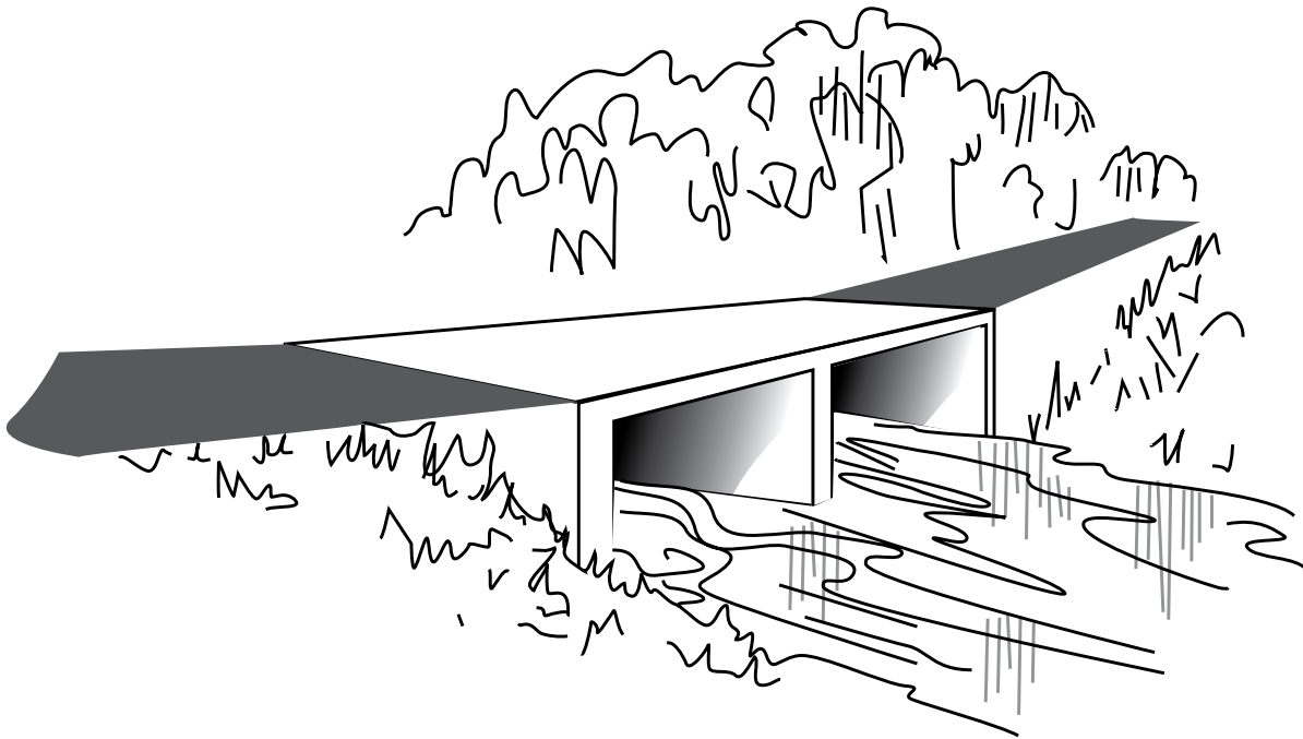
Figure 3.3-4. Concrete vented ford - The number of box openings depends upon the width and flow of the channel. A continuous streambed maintains channel function.
