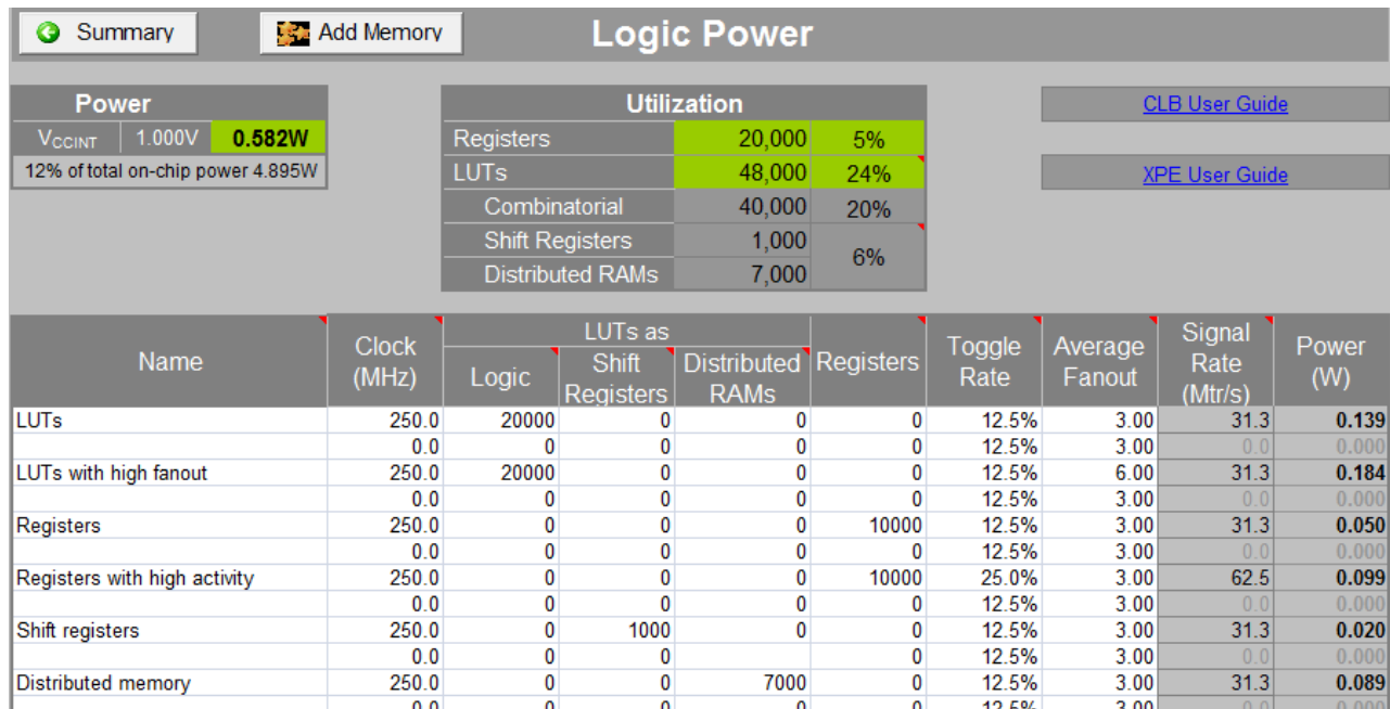
Figure 3-1: Effect of LUT Configuration, Toggle Rates, and Average Fanout on Power Estimation (7 Series Devices)
