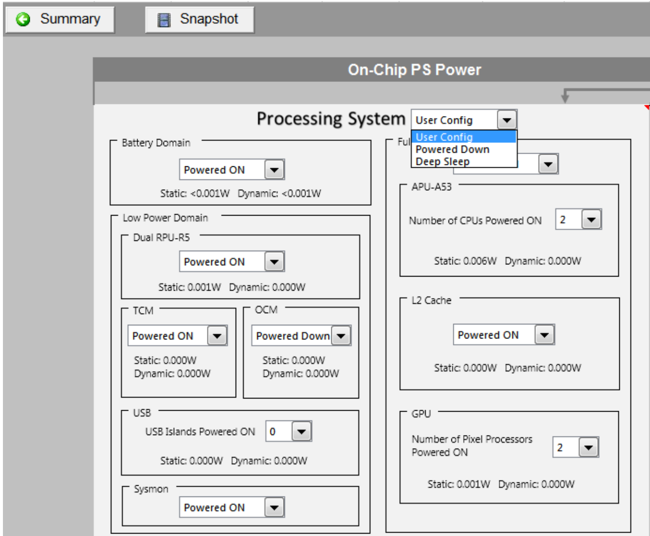
Figure 3-18: PS Sheet for Zynq UltraScale+ MPSoC displaying Input panel
