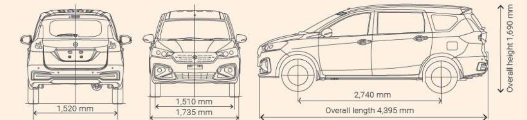
The drawings shown are general specifications of the vehicle.
