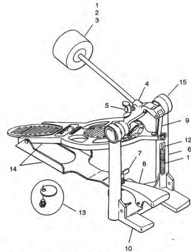
No. L-201 Speed King Pedal
