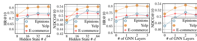
Figure 6: Hyper-parameter study of KCGN
