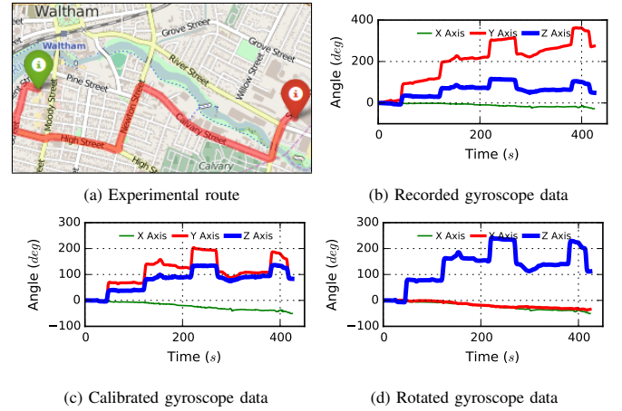
Fig. 4: Error compensation steps for gyroscope data.
