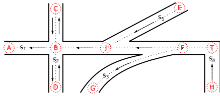
(a) Connections are created when a road bisects (B), furcates (F), joins (J) with another road, or turns (T) into a different direction. Created atomic parts: \overrightarrow{BA} , \overrightarrow{BC} , \overrightarrow{BD} , \overrightarrow{CB} , \overrightarrow{DB} , \overrightarrow{JG} , \overrightarrow{EJ} , \overrightarrow{FJ} , \overrightarrow{FG} , \overrightarrow{TF} , \overrightarrow{HT} .
