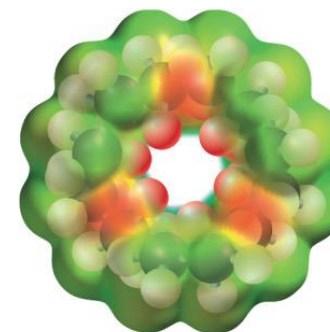
EPM of 18-crown-6
