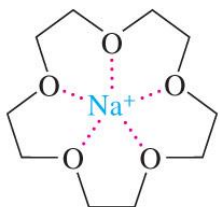
15-crown-5 solvates \text{Na}^+
