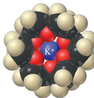
18-crown-6 with \text{K}^+ solvated
