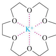
18-crown-6 solvates \text{K}^+
