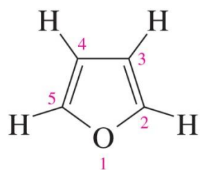
furan
