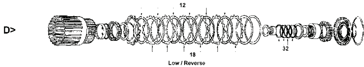
Low / Reverse
