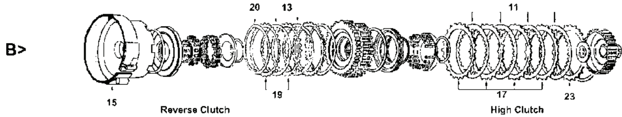
Reverse Clutch
