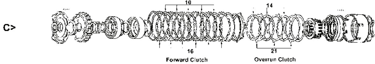
Forward Clutch
