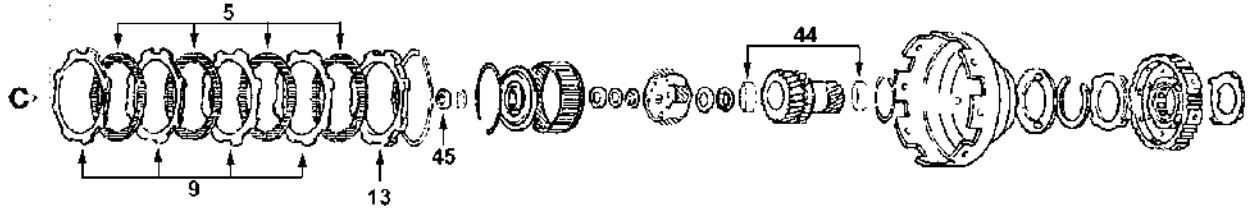
Forward Clutch
