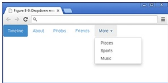
Figure 8-9: Bootstrap toolbar with drop-down menus.
