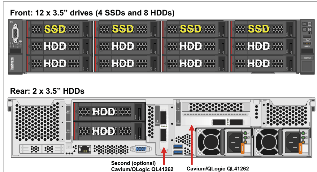
Figure 42 Lenovo ThinkSystem SR650 storage subsystem configured for iWARP
