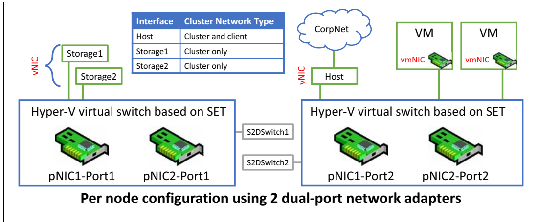
Figure 53 Diagram showing two SET teams created from two dual-port network adapters
