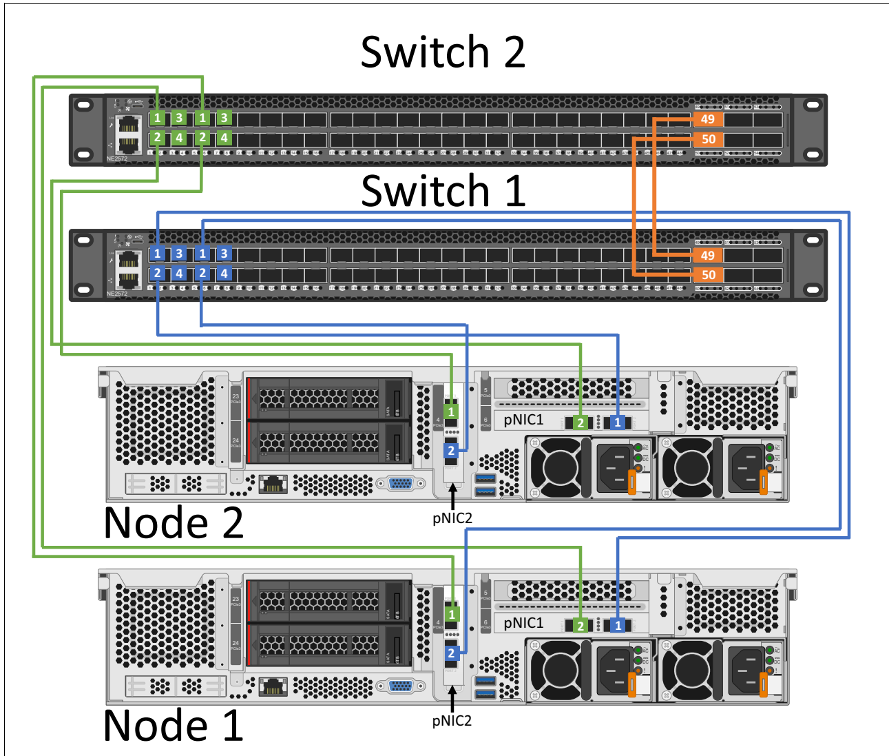
Figure 46 Switch to node connectivity using 10GbE / 25GbE AOC / DAC cables and two dual-port NICs in each node
