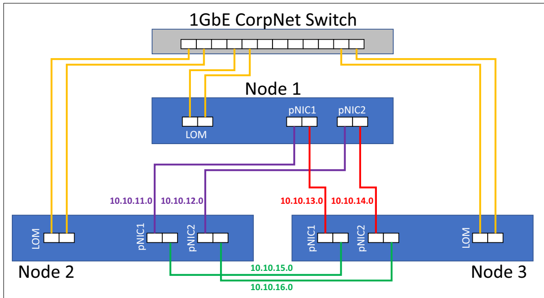
Figure 60 Three-node connectivity for direct-connected deployment scenario
