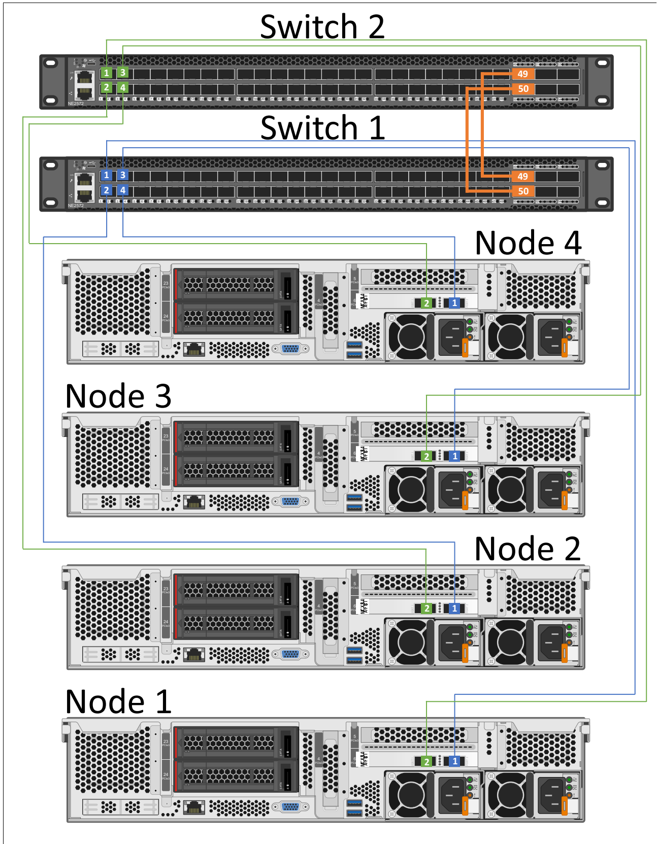
Figure 45 Switch to node connectivity using 10GbE / 25GbE AOC / DAC cables and a single dual-port NIC in each node
