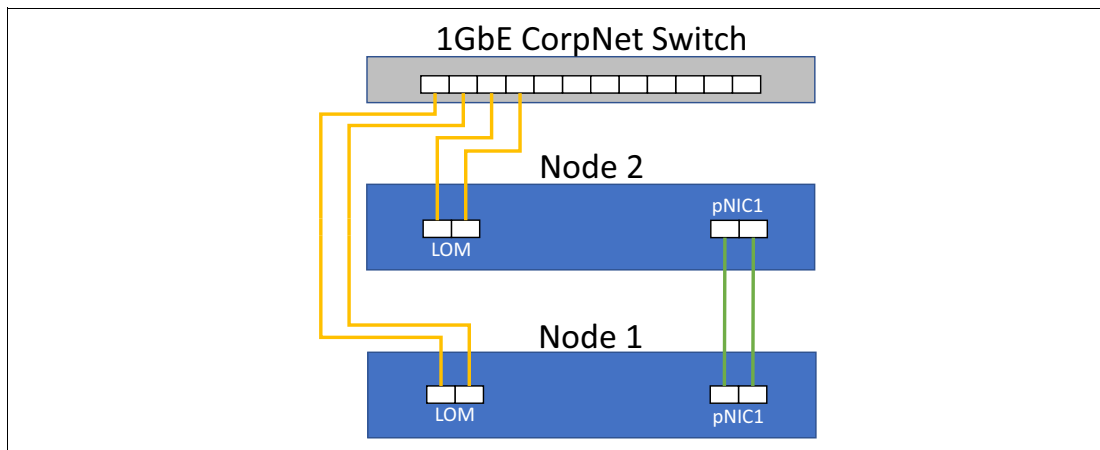
Figure 59 Two-node connectivity for direct-connected deployment scenario
