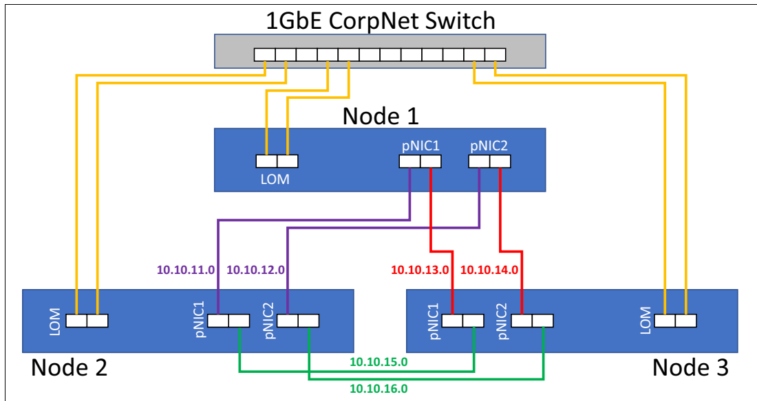
Figure 35 Three-node connectivity for direct-connected deployment scenario
