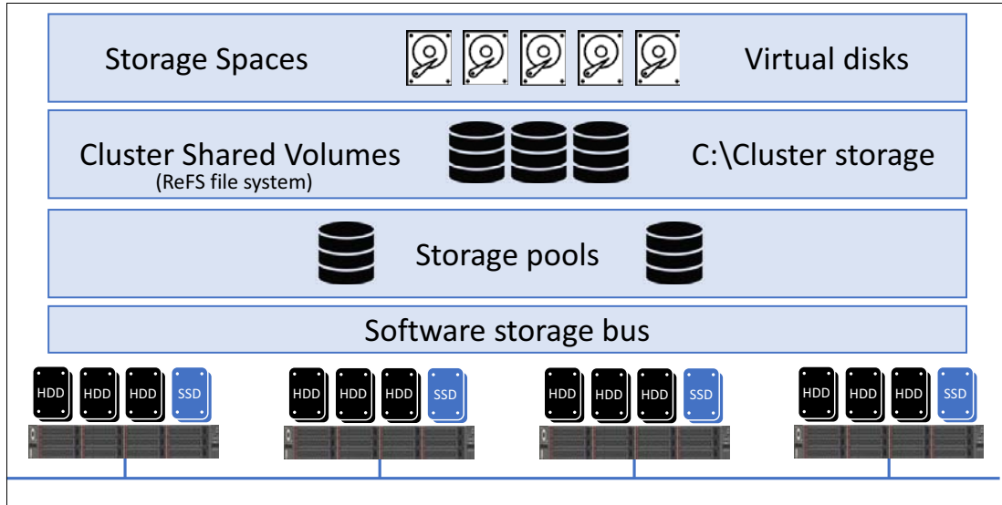
Figure 2 Converged/disaggregated S2D deployment type - nodes do not host VMs
