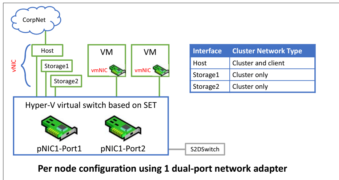
Figure 49 Diagram showing single SET team created from both ports on a single network adapter
