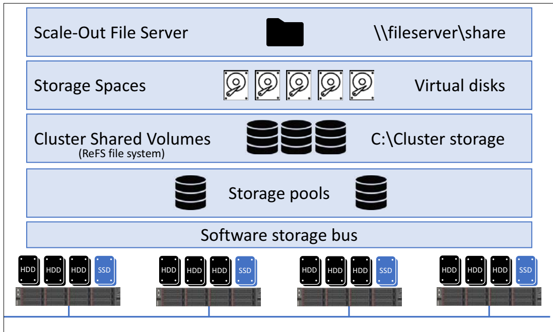
Figure 1 Storage Spaces Direct stack
