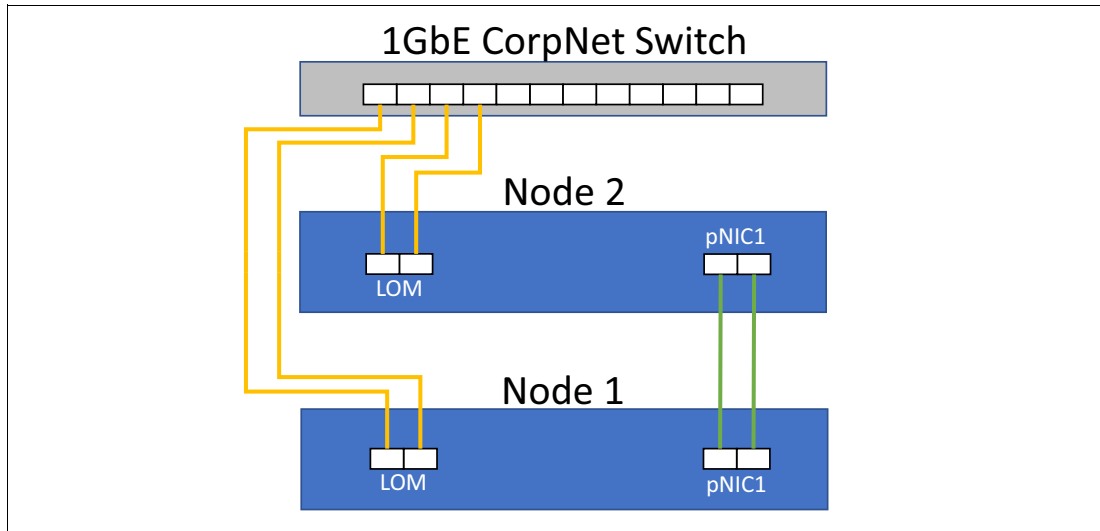
Figure 34 Two-node connectivity for direct-connected deployment scenario
