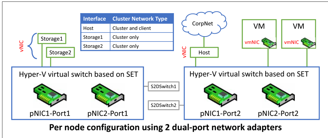
Figure 28 Diagram showing two SET teams created from two dual-port network adapters
