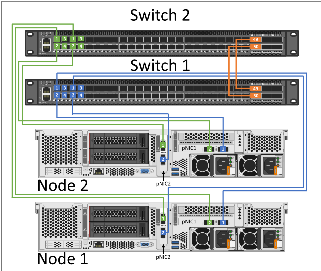
Figure 23 Switch to node connectivity using 10GbE / 25GbE AOC / DAC cables and two dual-port NICs in each node
