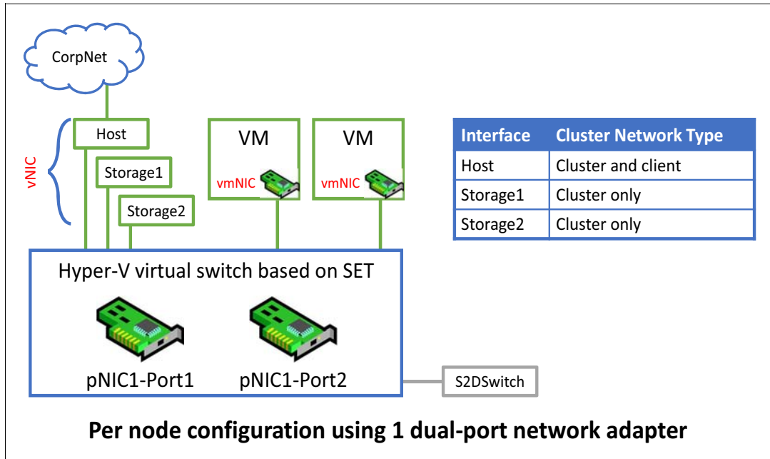
Figure 24 Diagram showing single SET team created from both ports on a single Mellanox NIC
