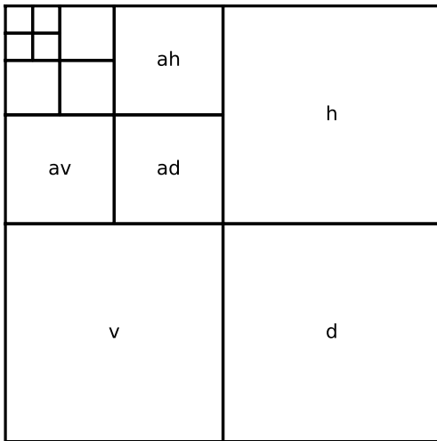
wavedec2 (4 level)
