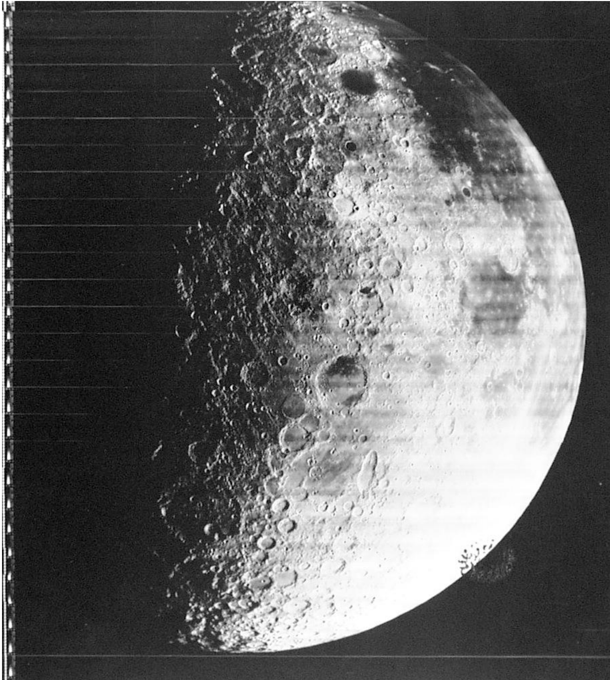
Figure 3 - Grimaldi crater
